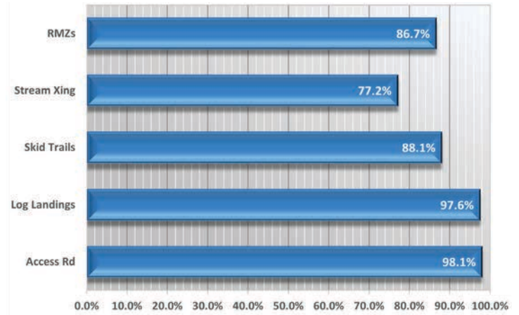
Figure 8. Overall BMP effectiveness for each of the five BMP categories.
