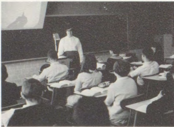
The square of the hypotenuse is equal to .....
