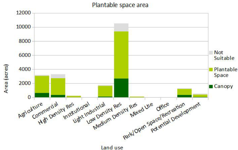
Fig 6: Low density residential has the greatest potential for increasing the canopy, followed by commercial.
