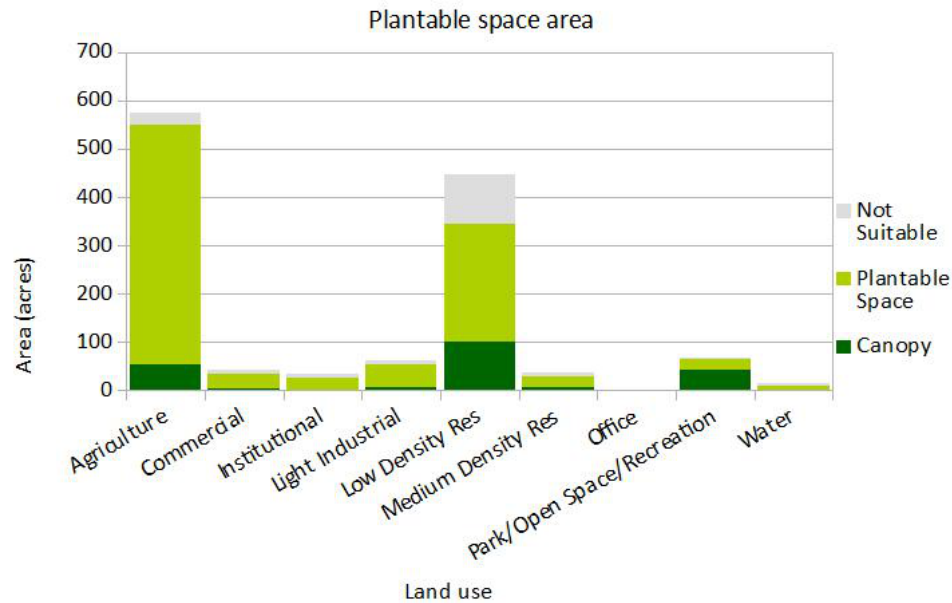
Fig 6: Agriculture has the greatest potential for increasing the canopy, followed by residential properties.
