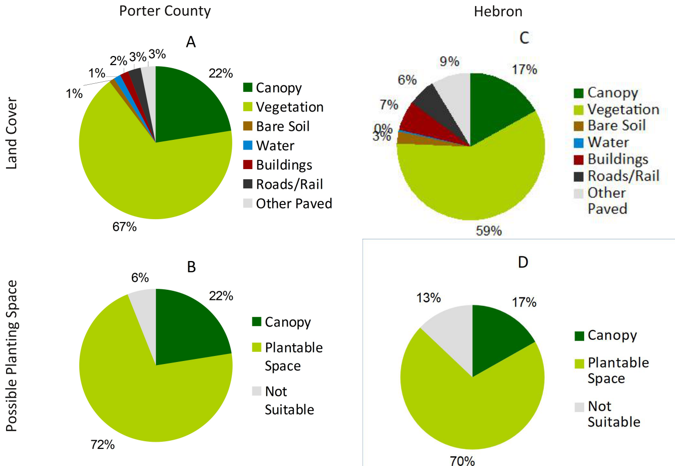
Fig 2: Porter County's current land cover (A), including 22% canopy cover. An additional 72% of the county is suitable for planting (B). Hebron currently has 17% canopy cover (C), and 70% of the land cover could potentially be converted to canopy (D).
