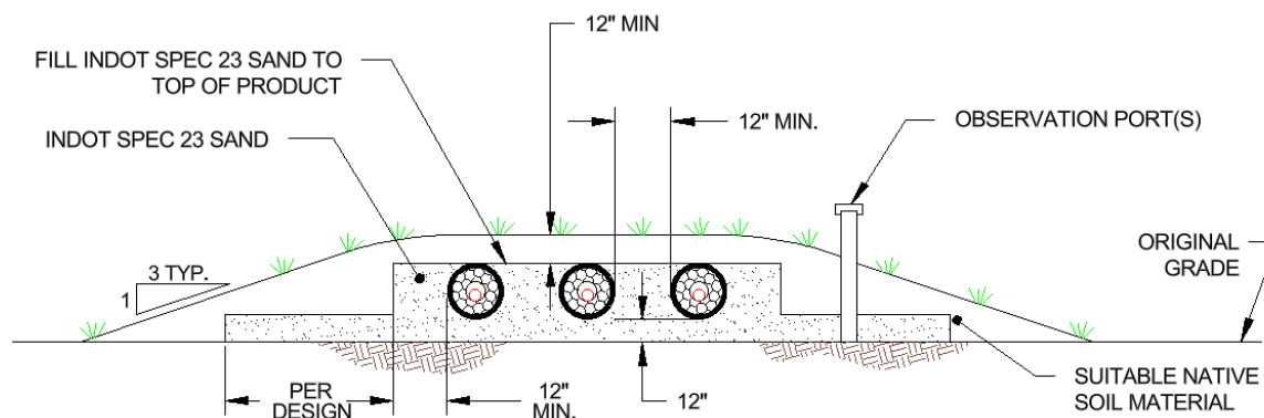
Figure 1.1. ATL with pressure distribution cross section.
