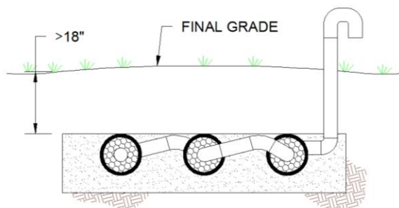
Vent cross-section for all applications when greater than 18" of cover material is placed atop the ATL System.
