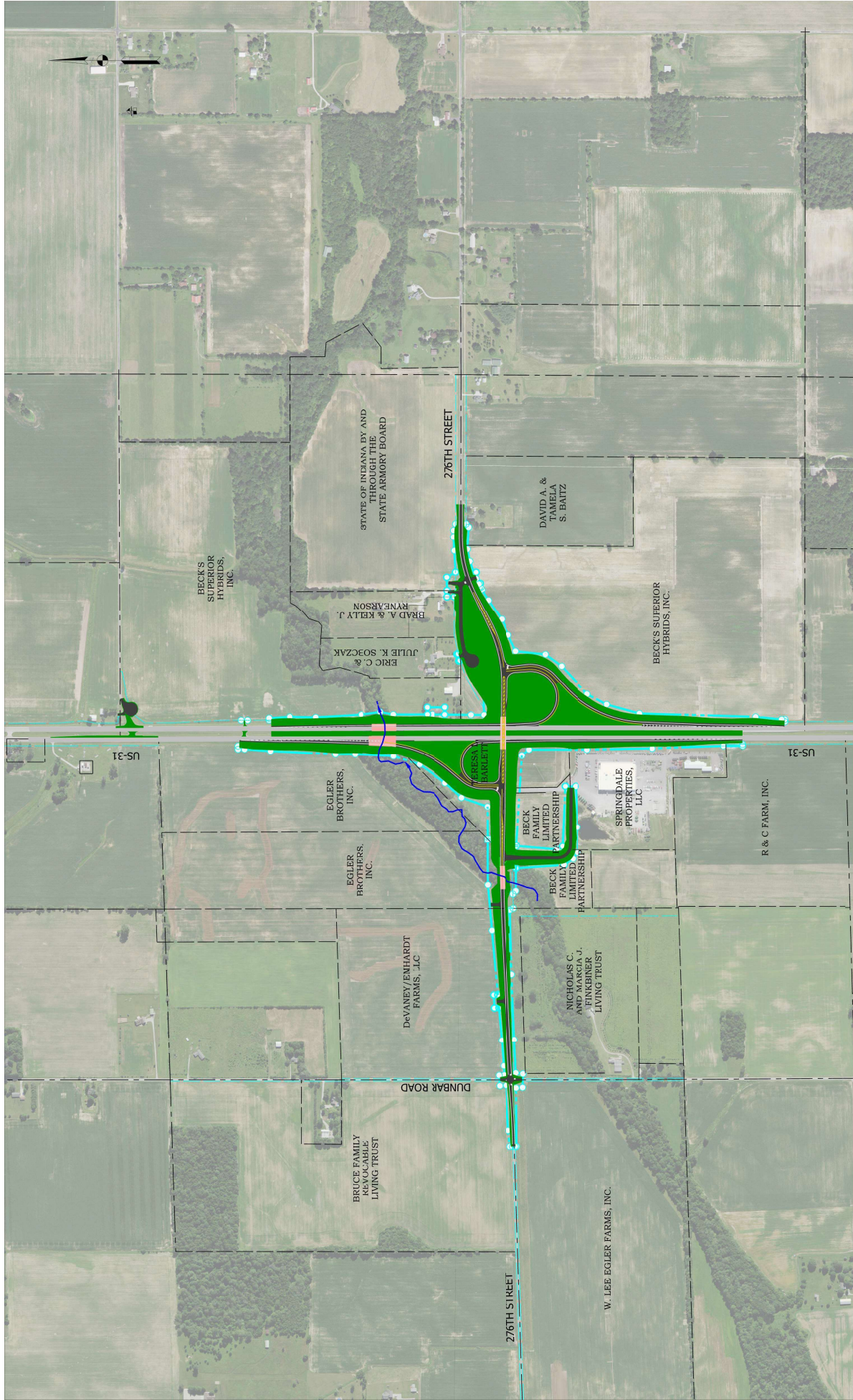
US 31 New Interchange (Des No. 1901797) - Hamilton County, IN Preliminary Preferred Alternative - Alternative 1
