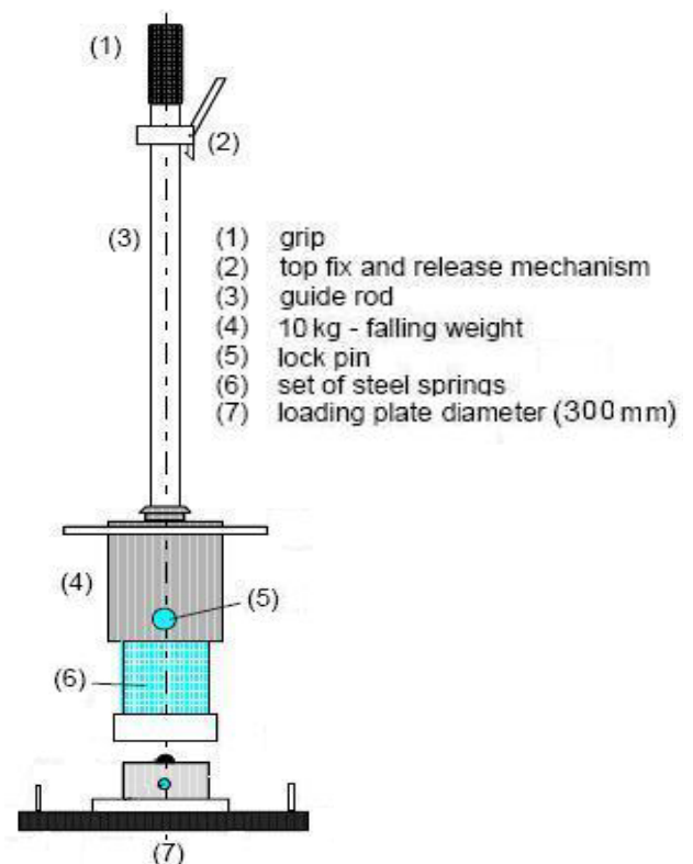
Figure 12-2 Breakdown of an LWD
