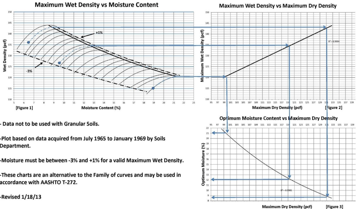
Figure 14-1 Typical Moisture Density Curves
