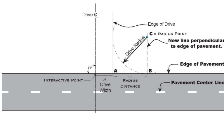
Figure 7-1 Radius Layout for Square Drive/Approach
