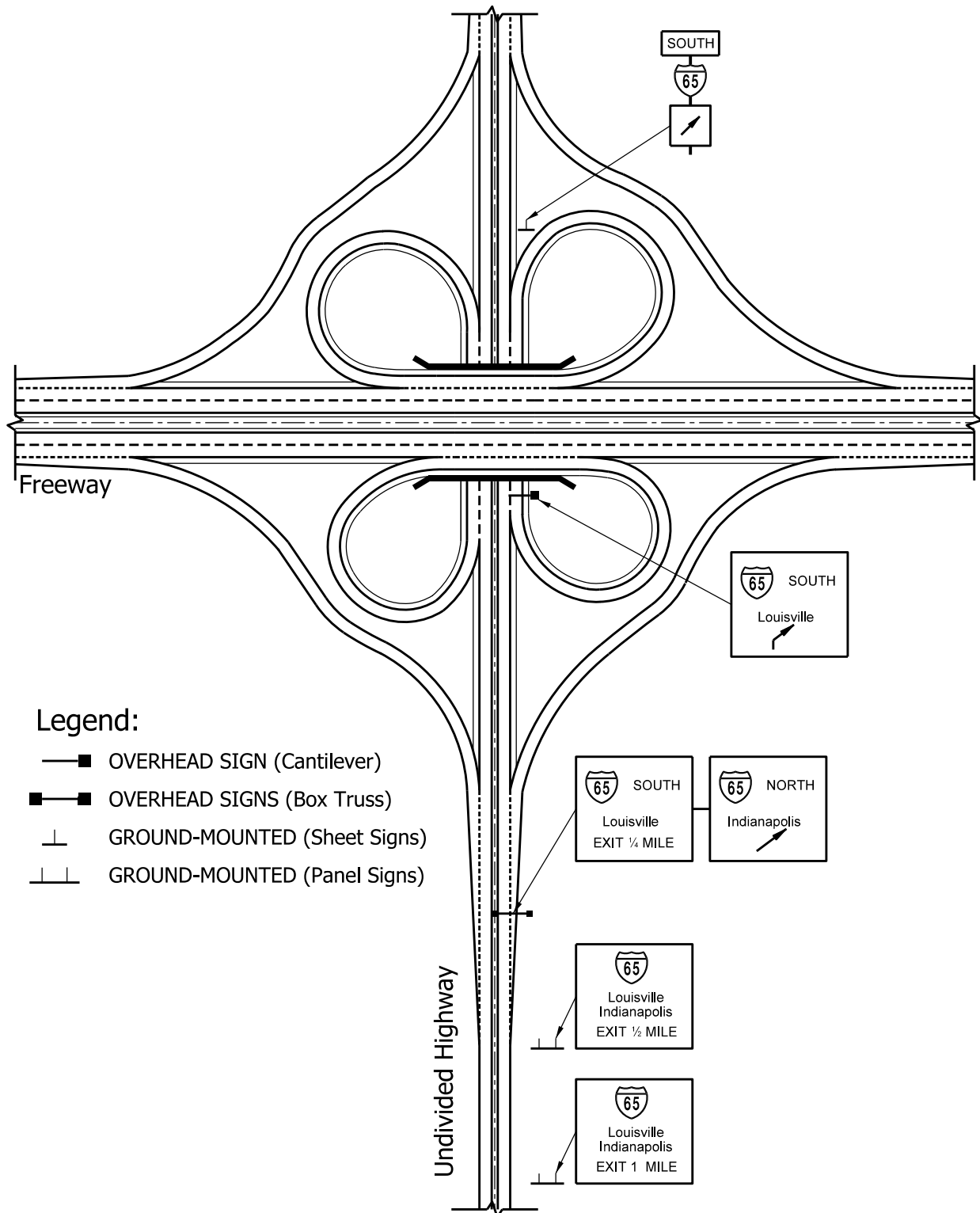
FULL CLOVERLEAF INTERCHANGE SIGNING (Freeway over Undivided Highway)
