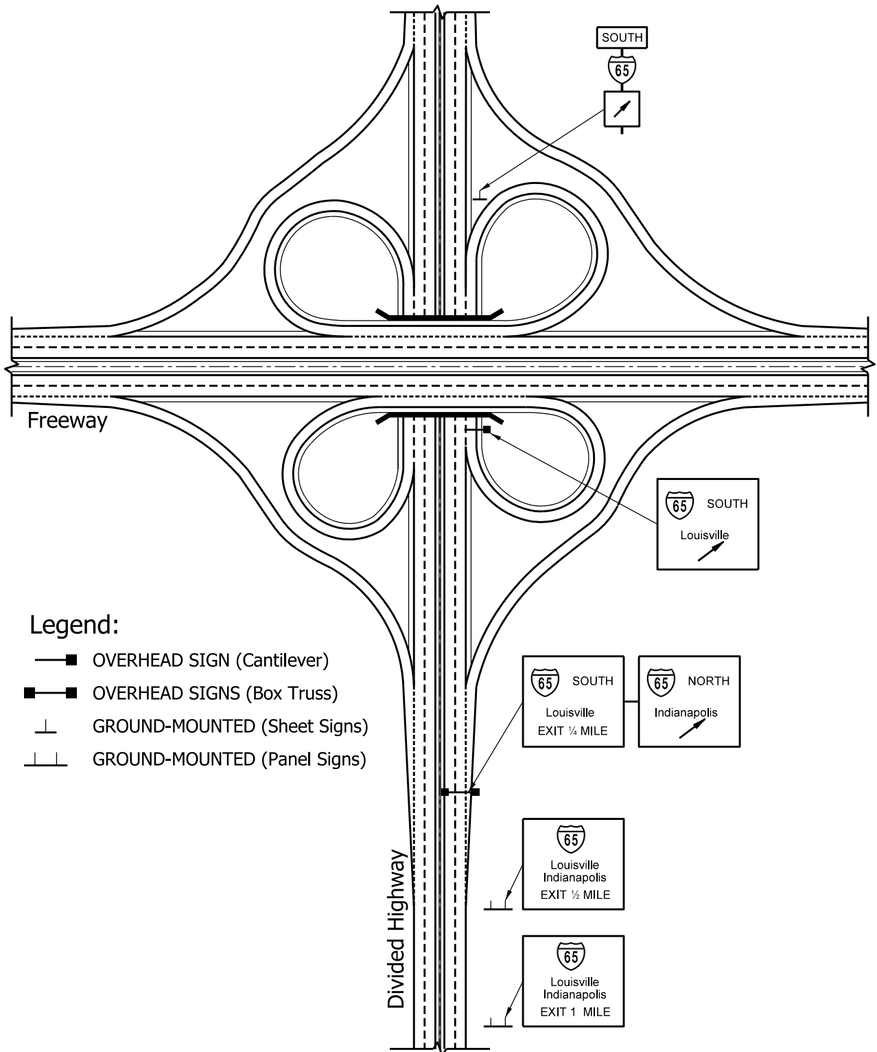
FULL CLOVERLEAF INTERCHANGE SIGNING (Freeway over Divided Highway)
