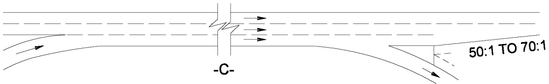
-C- AUXILIARY LANE DROPPED AT PHYSICAL NOSE
