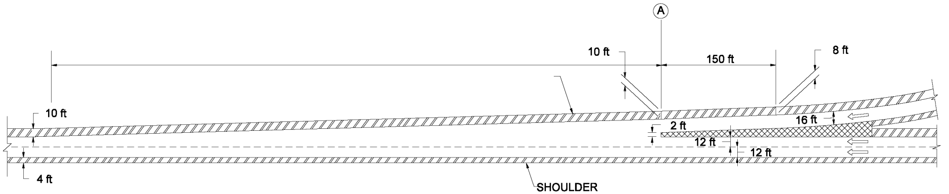
PARALLEL DESIGN (PREFERRED)
