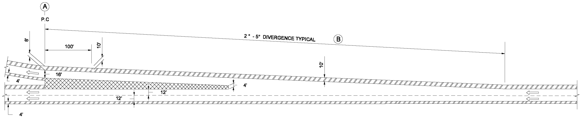
TAPERED DESIGN
