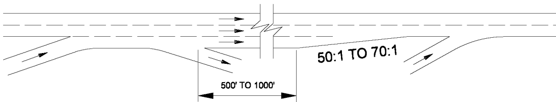
-D- AUXILIARY LANE DROPPED WITHIN AN INTERCHANGE
