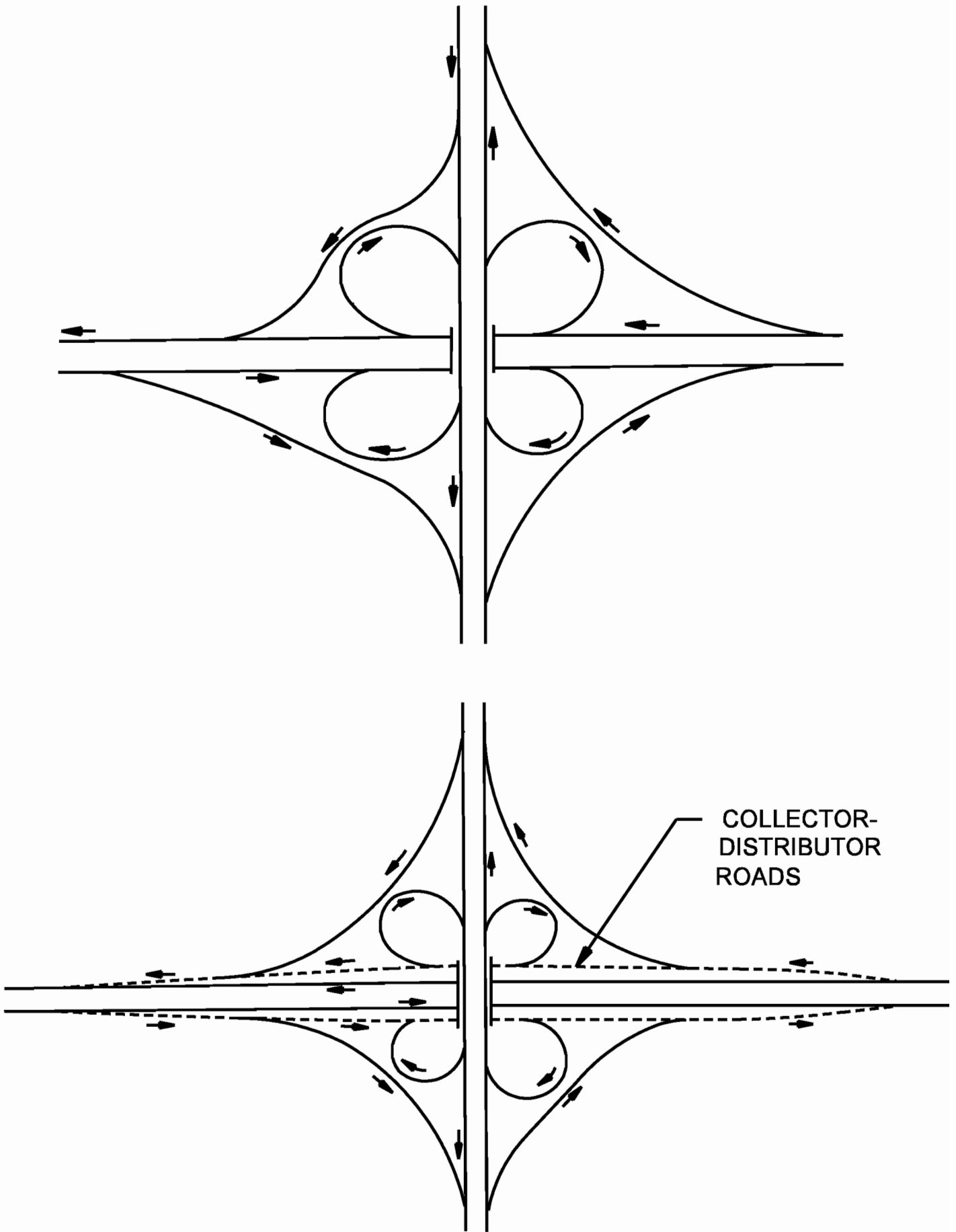
FULL CLOVERLEAFS
