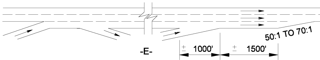
-E- AUXILIARY LANE DROPPED BEYOND AN INTERCHANGE
