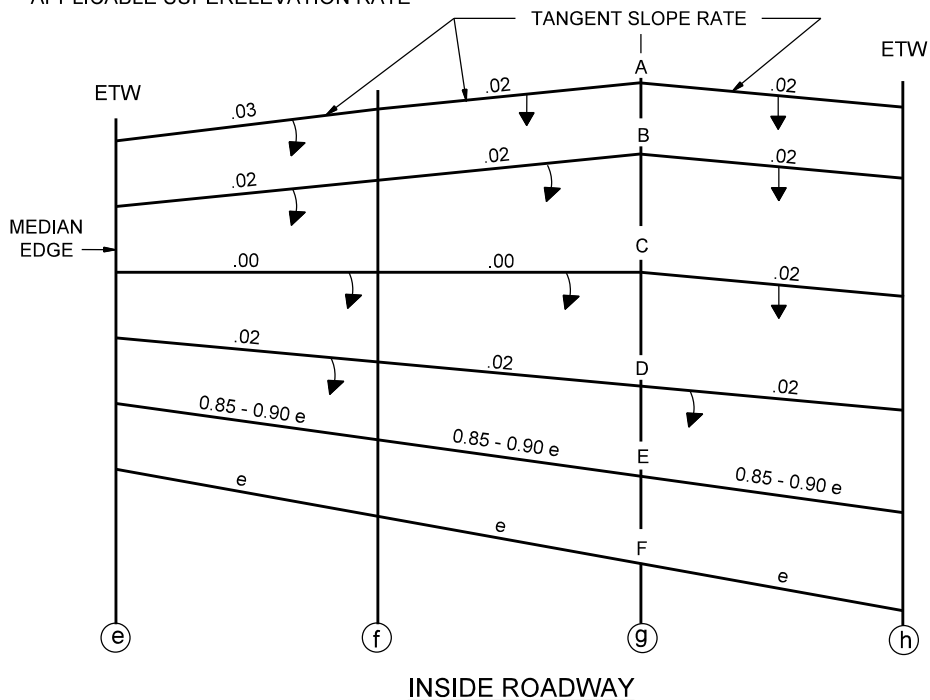
SUPERELEVATION DEVELOPMENT (Six-Lane (or more) Divided) (Four-Lane Divided with Future Additional Lanes)
