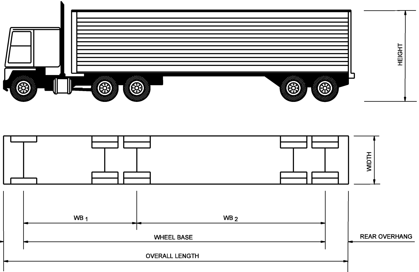
BASIC DIMENSIONS OF DESIGN VEHICLE (Combination Truck A)
