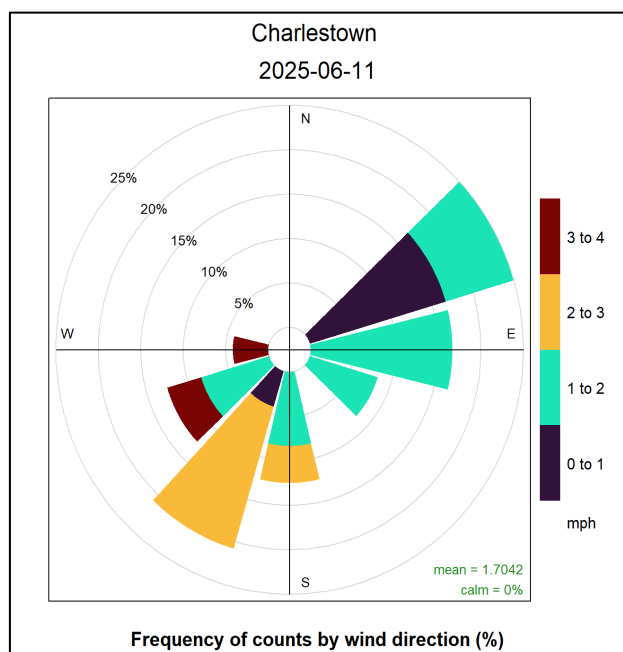
Figure 3.3.3 – Charlestown Windrose
