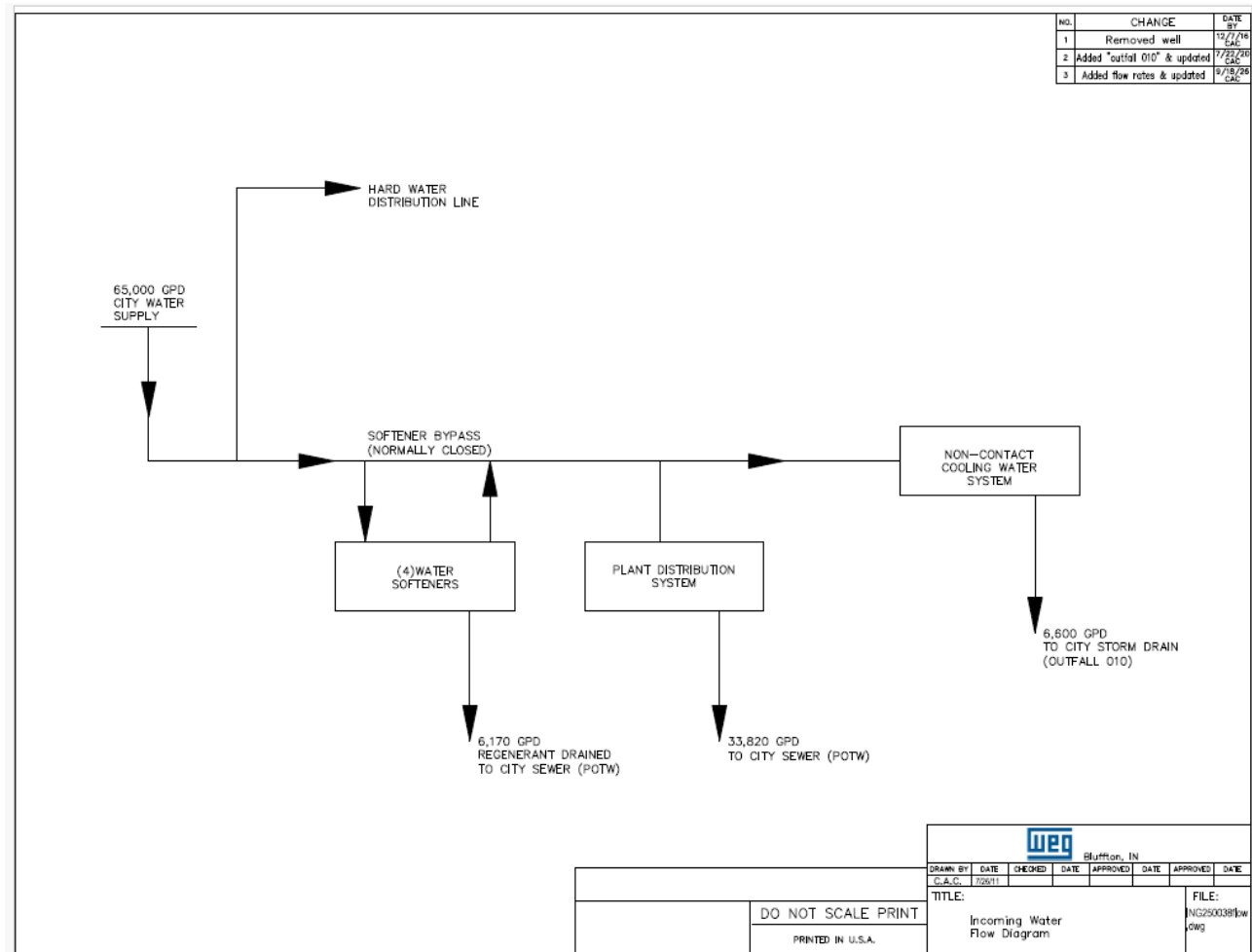
Figure 1a: Incoming Water Flow Diagram
