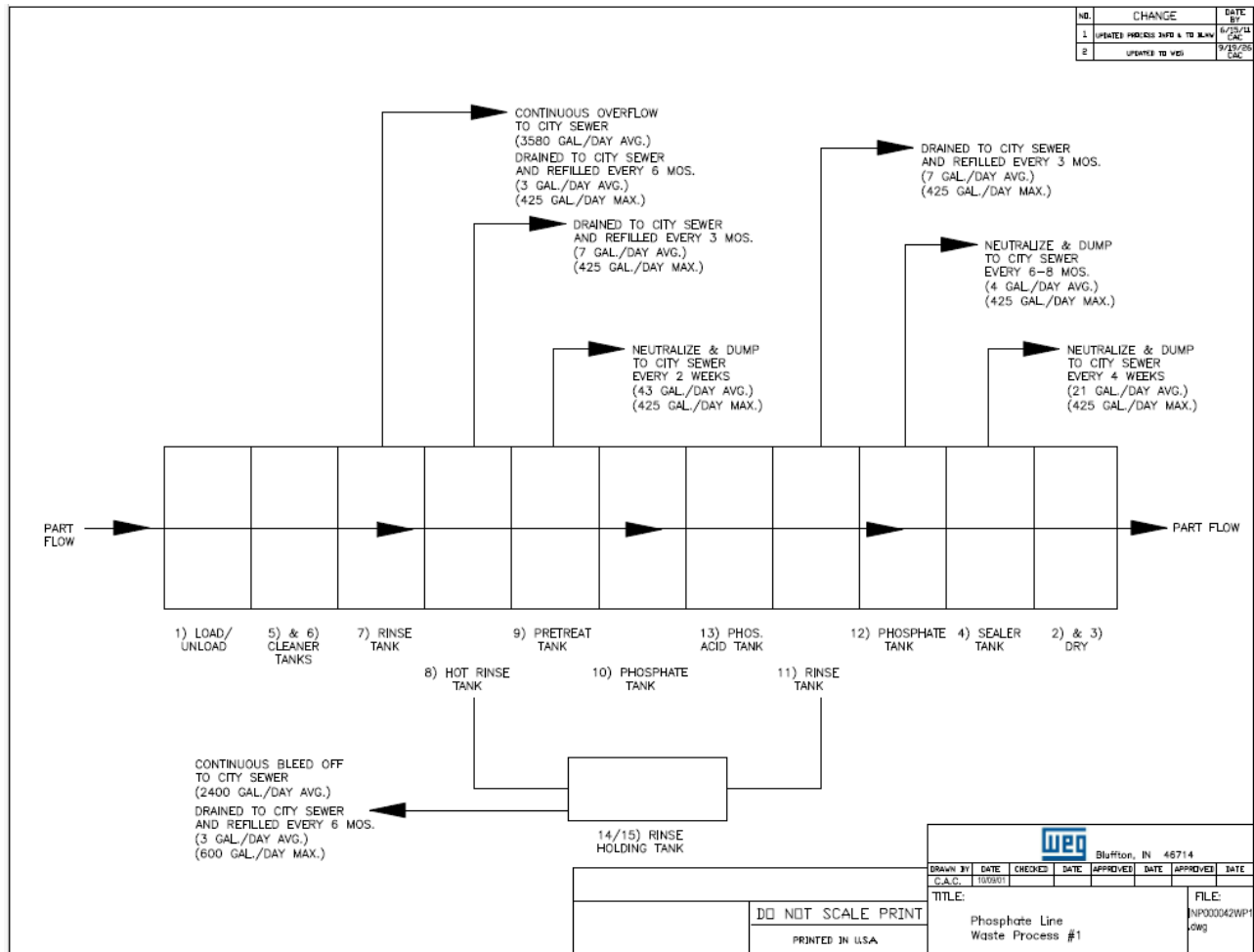
Figure 1b: Phosphate Line Wastestream #1
