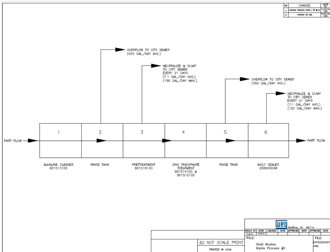
Figure 1c: Shell Washer Wastestream #2
