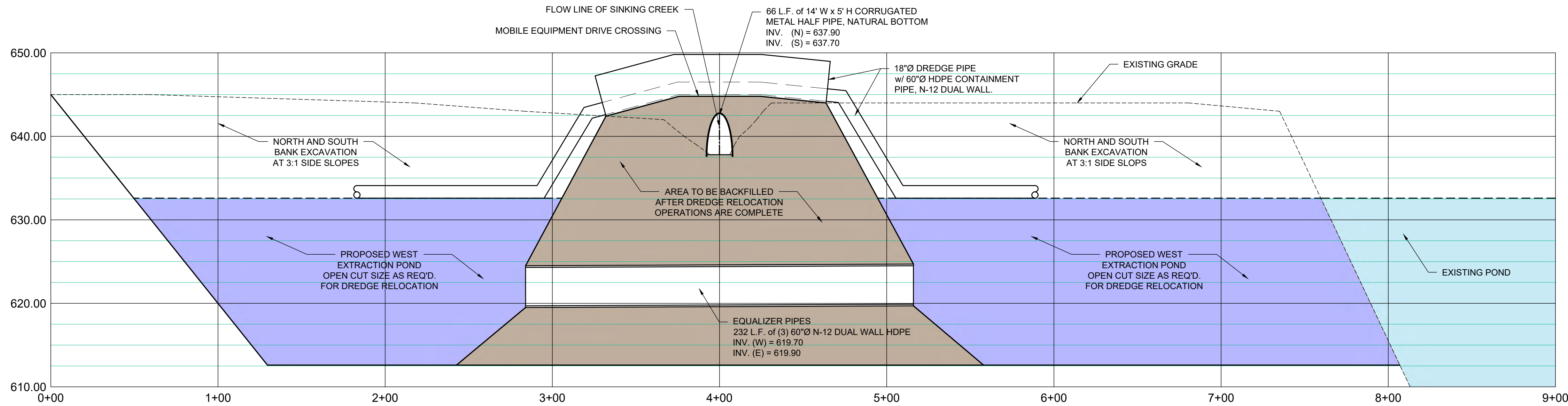
PERMANENT CROSSING - PERPENDICULAR TO SINKING CREEK (EAST-WEST)
