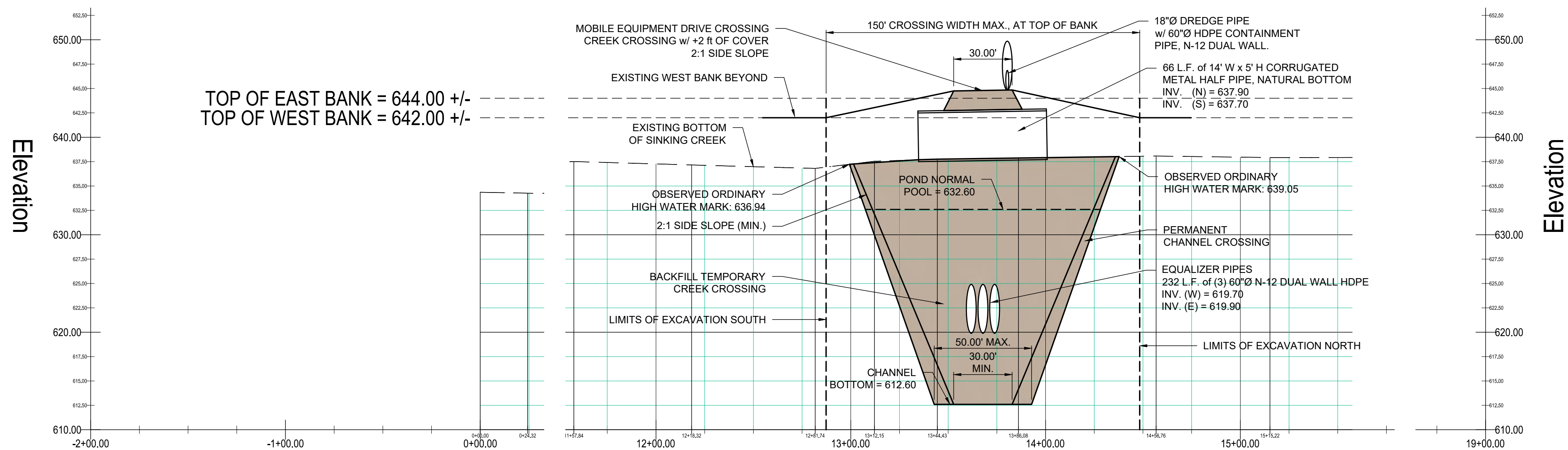
PERMANENT CROSSING (NORTH-SOUTH)
