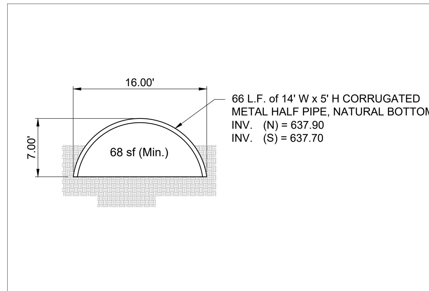
SINKING CREEK CULVERT DETAIL
