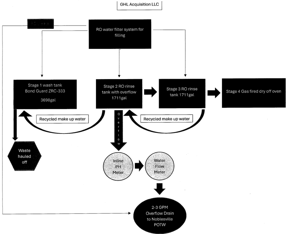
Figure 1: Flow Diagram
