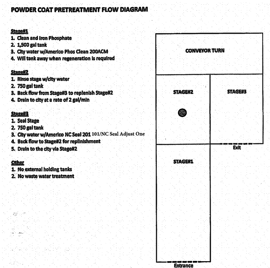
Figure 1: Flow Diagram
