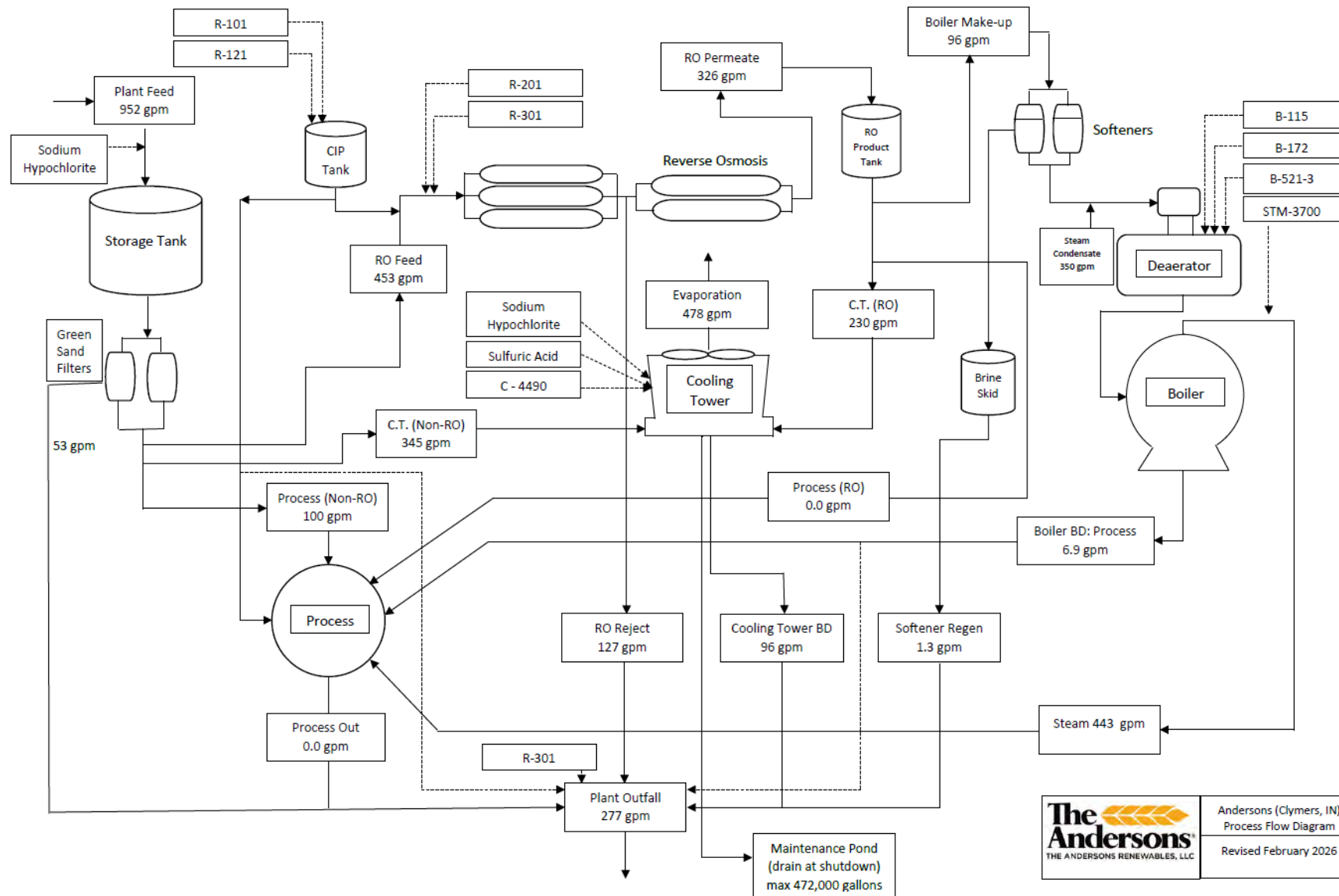
Figure 2: Water Balance Diagram
