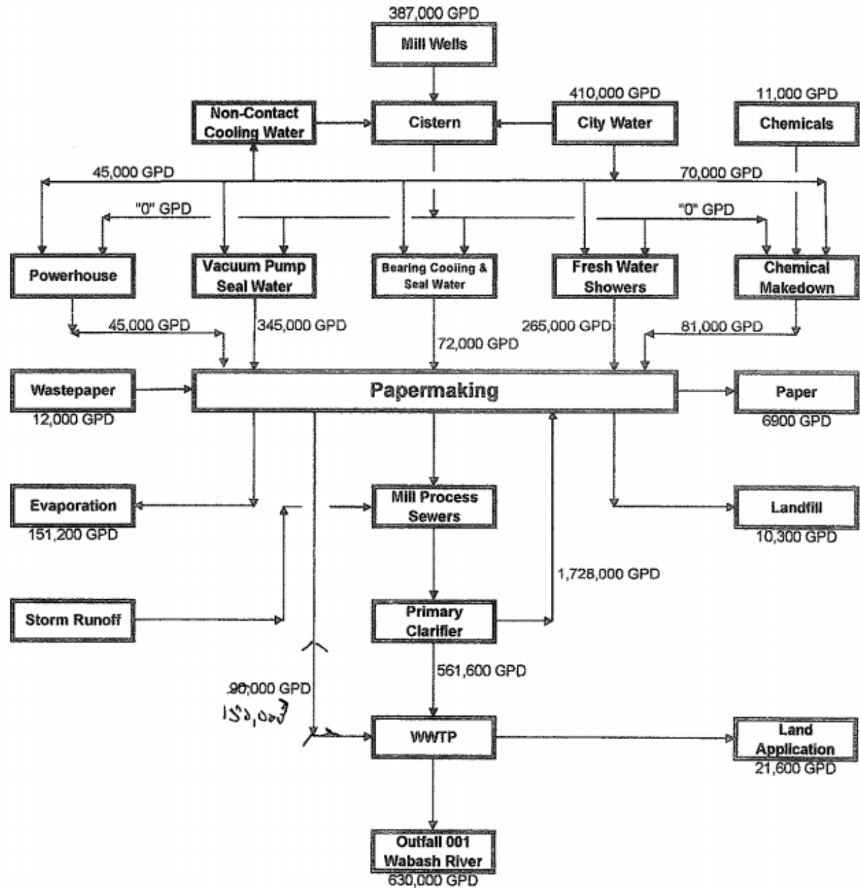
Figure 2: Water Balance Diagram
