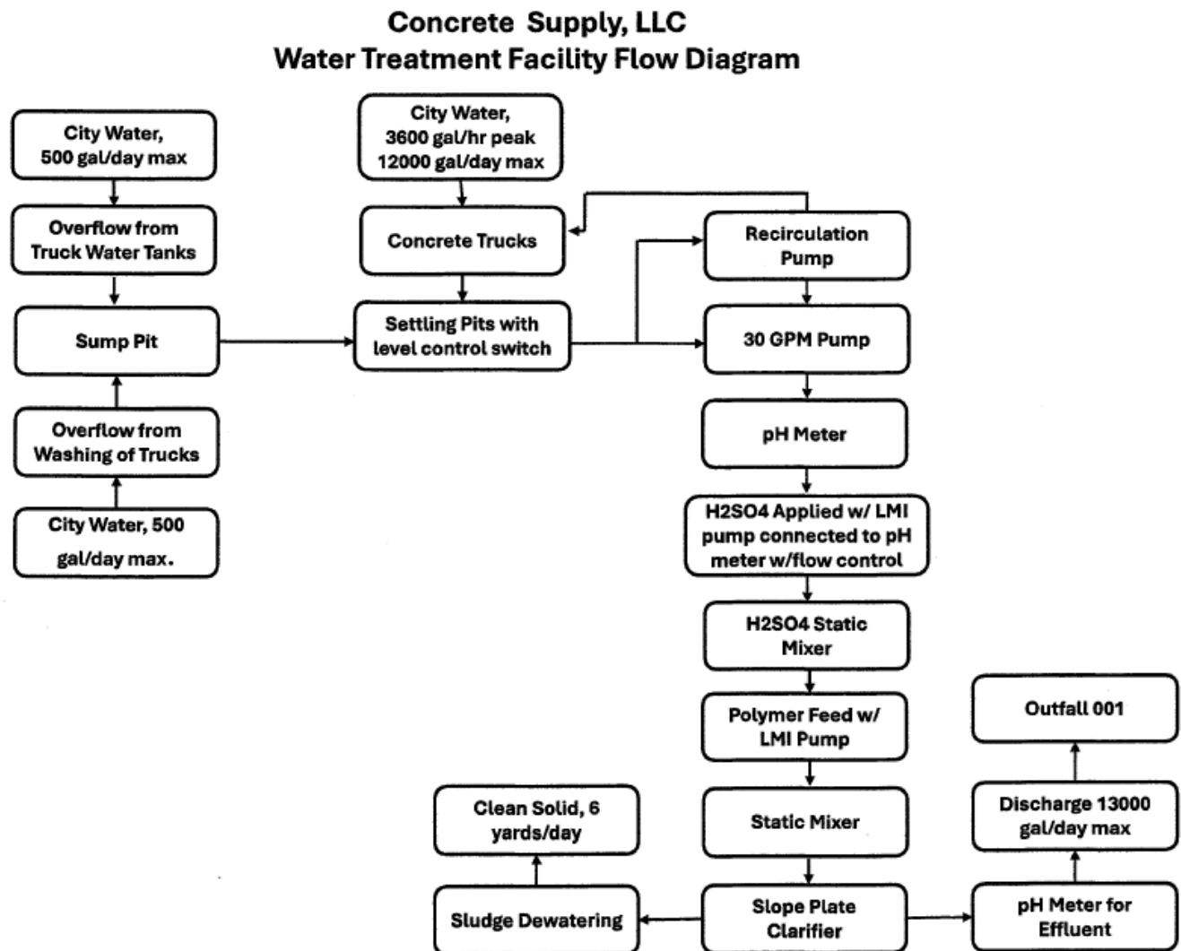
Figure 2: Water Balance Diagram
