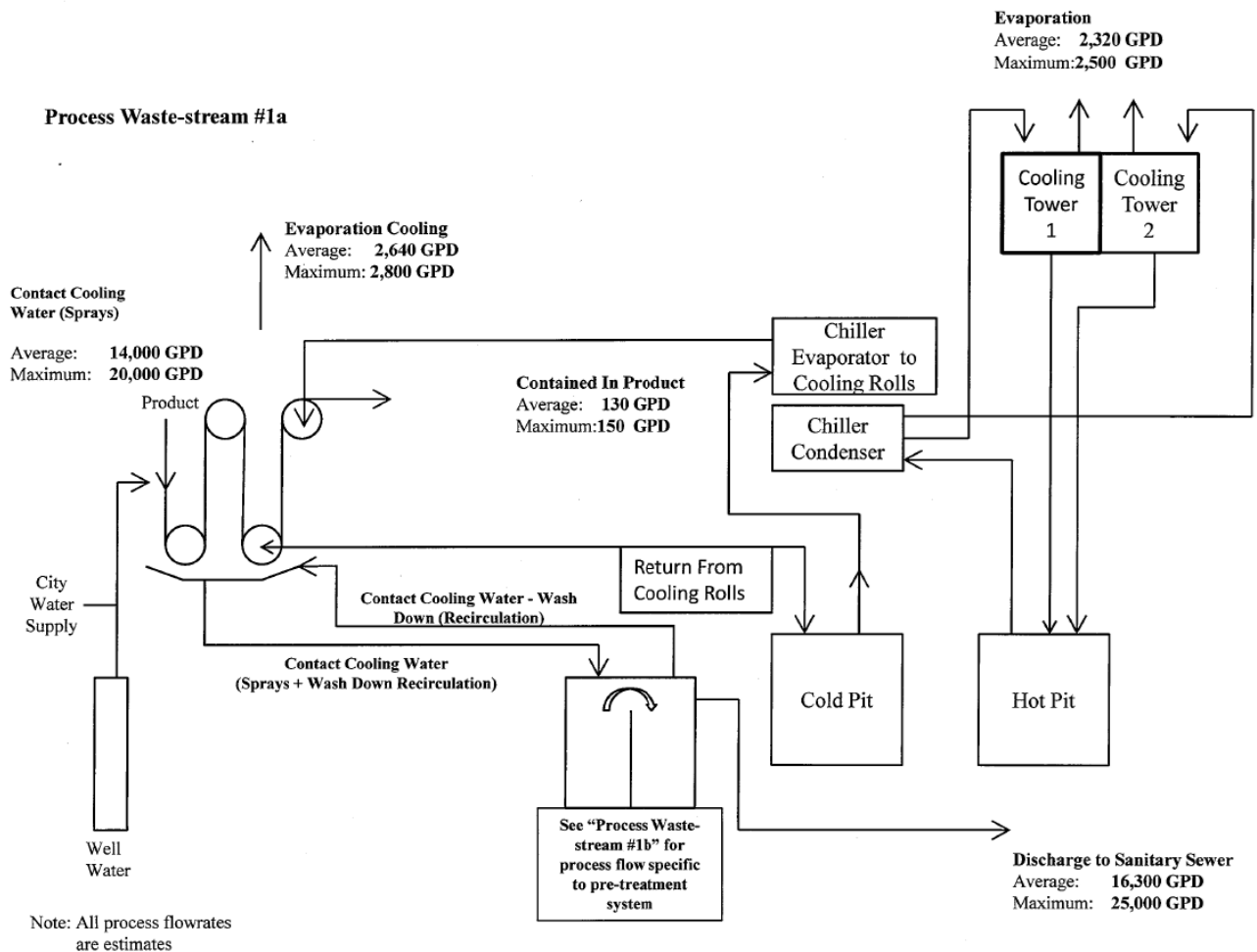
Figure 1: Process Wastestream #1 Flow Diagram
