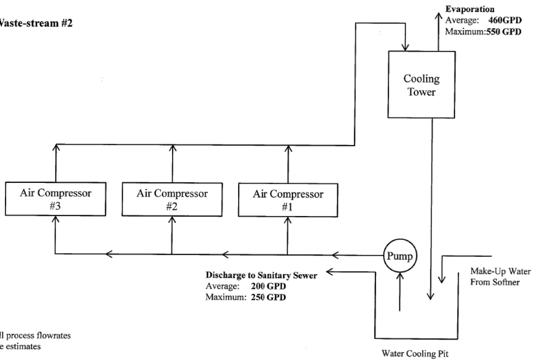
Figure 3: Non-Contact Cooling Waters Flow Diagram
