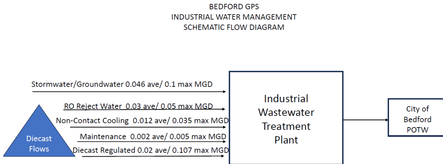
Figure 1: Flow Diagram
