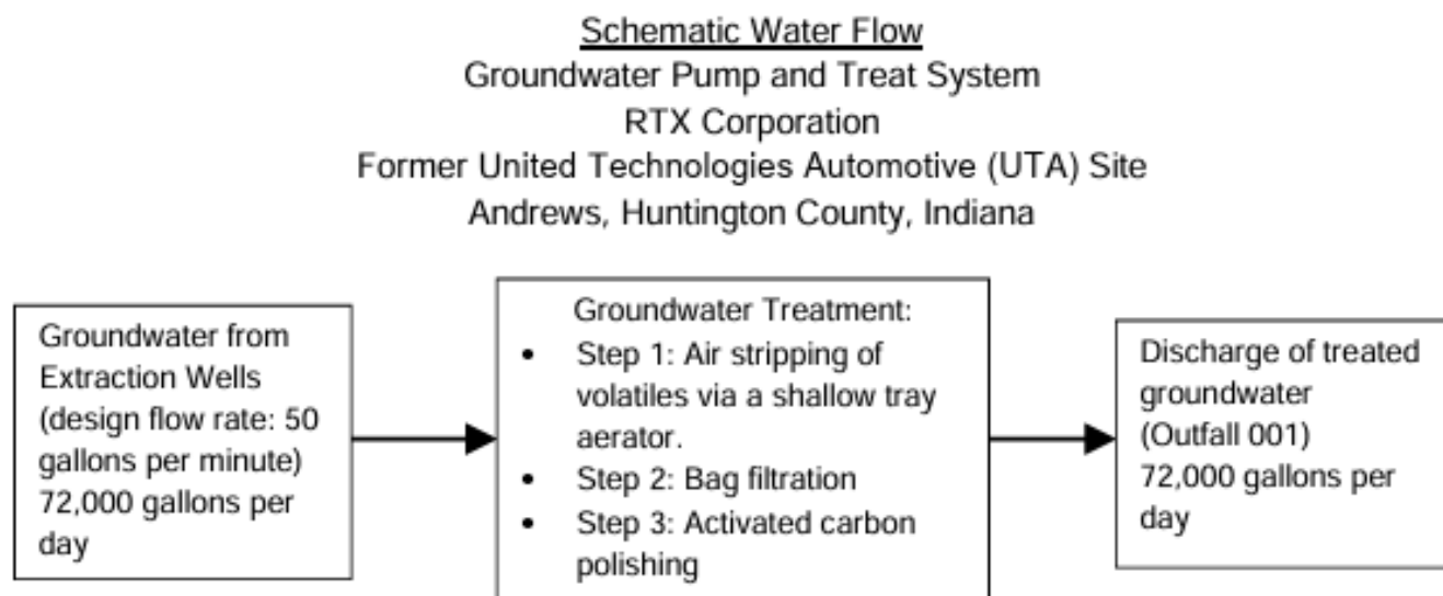
Figure 2: Water Balance Diagram
