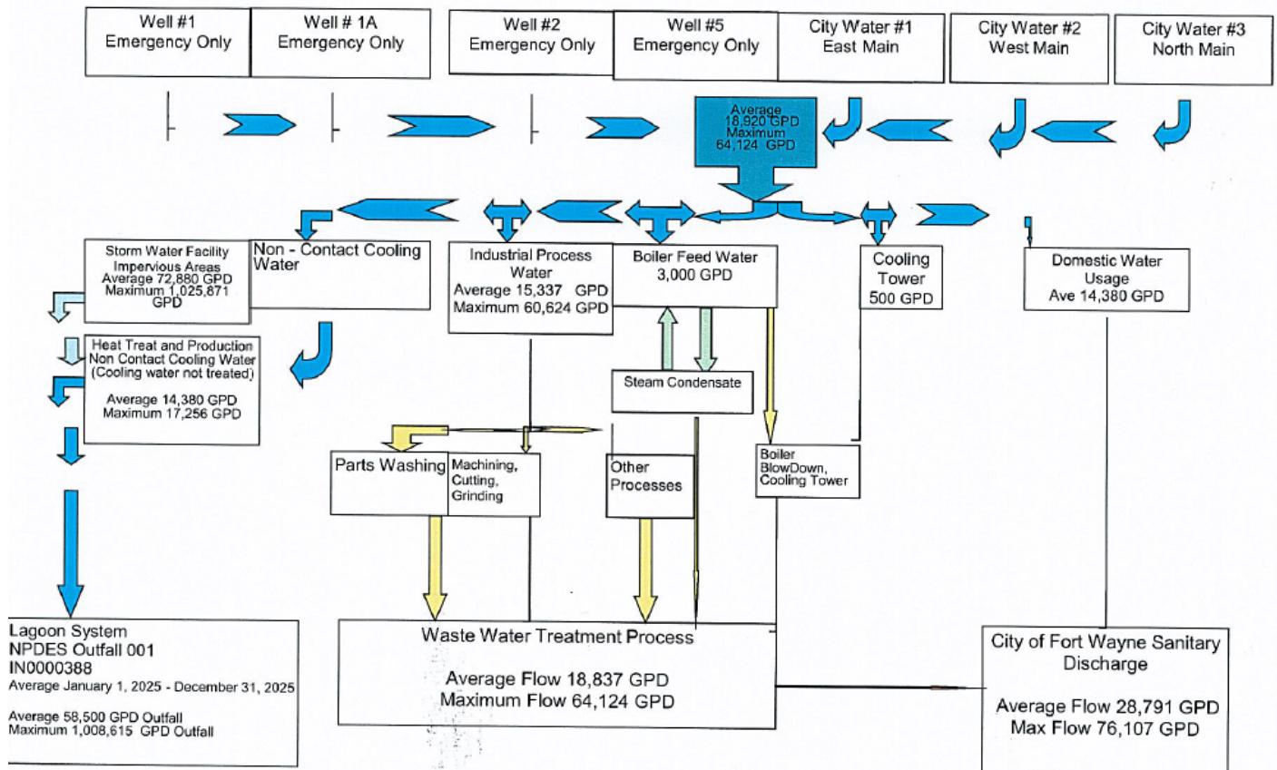
Figure 2: Water Balance Diagram
