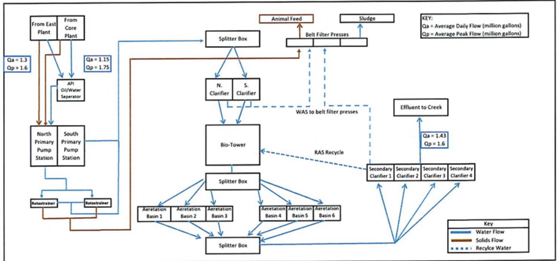
Figure 2: Water Balance Diagram
