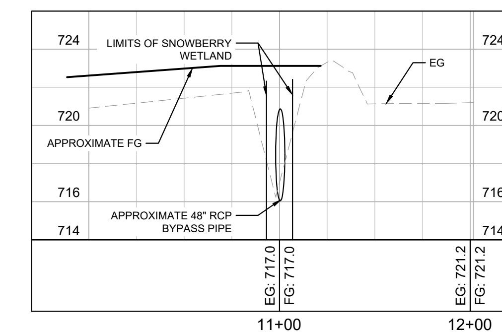
SNOWBERRY WETLAND CROSS-SECTION 01-01 V: 1" = 5' | H: 1" = 50'
