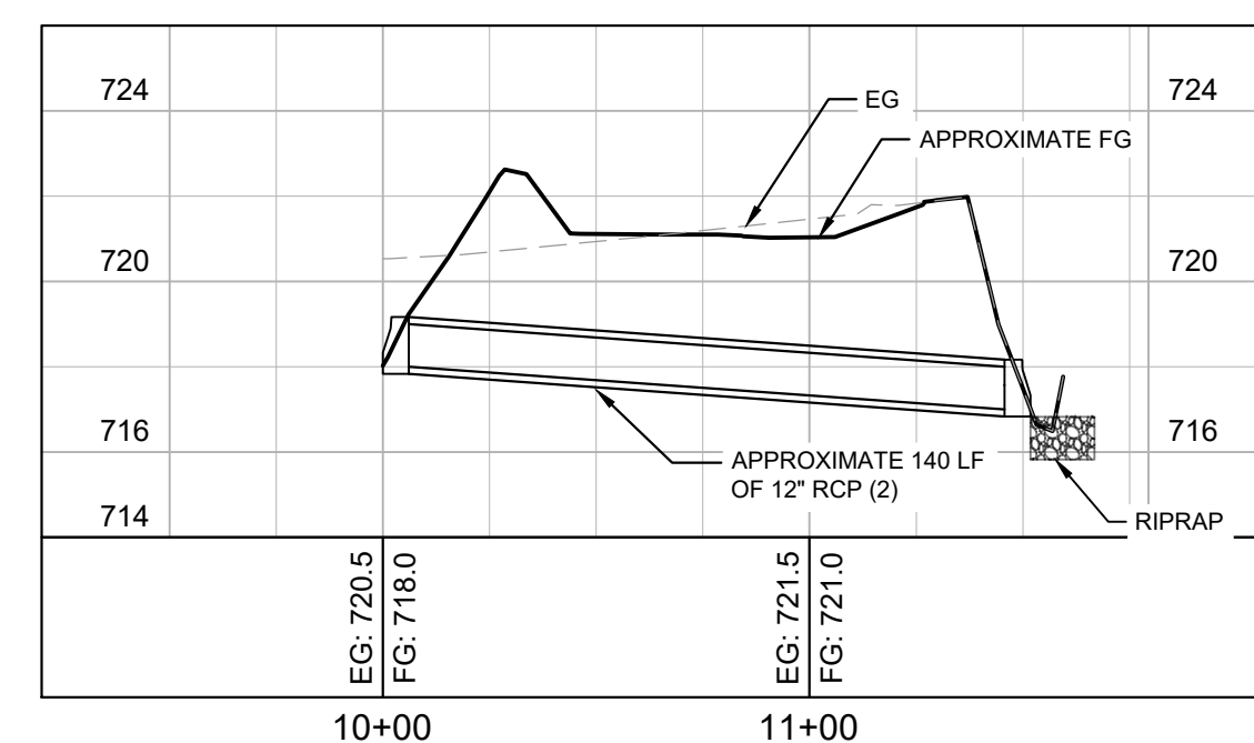
SNOWBERRY WETLAND OUTFALL V: 1" = 5' | H: 1" = 50'
