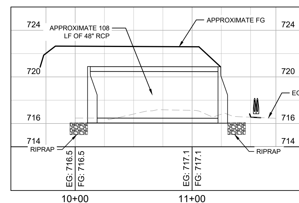
SNOWBERRY WETLAND CULVERT CROSSING V: 1" = 5' | H: 1" = 50'
