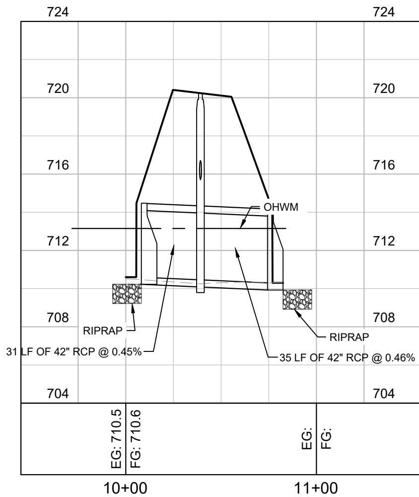
S1 STREAM A CULVERT CROSSING V: 1" = 5' | H: 1" = 50'
