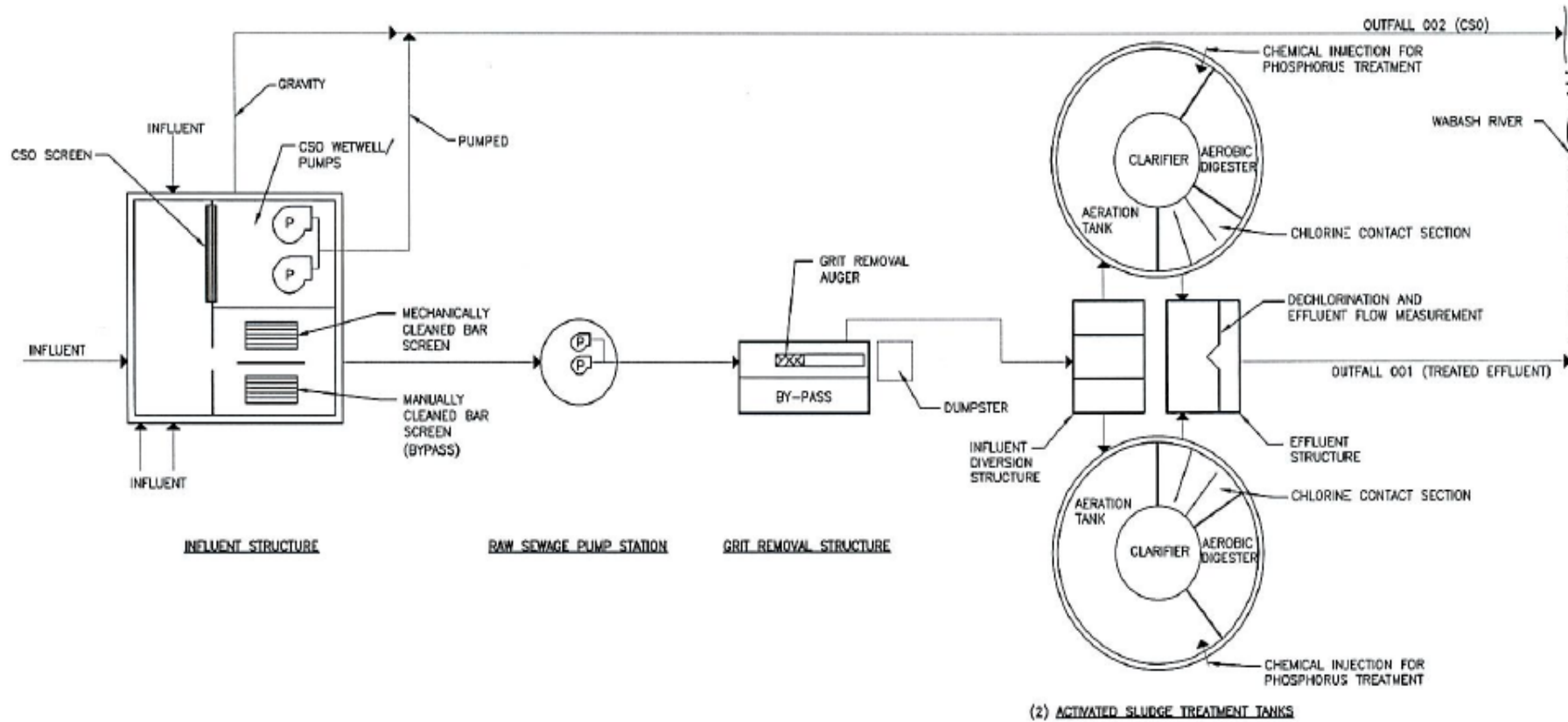
① WASTEWATER FLOW DIAGRAM NO SCALE
