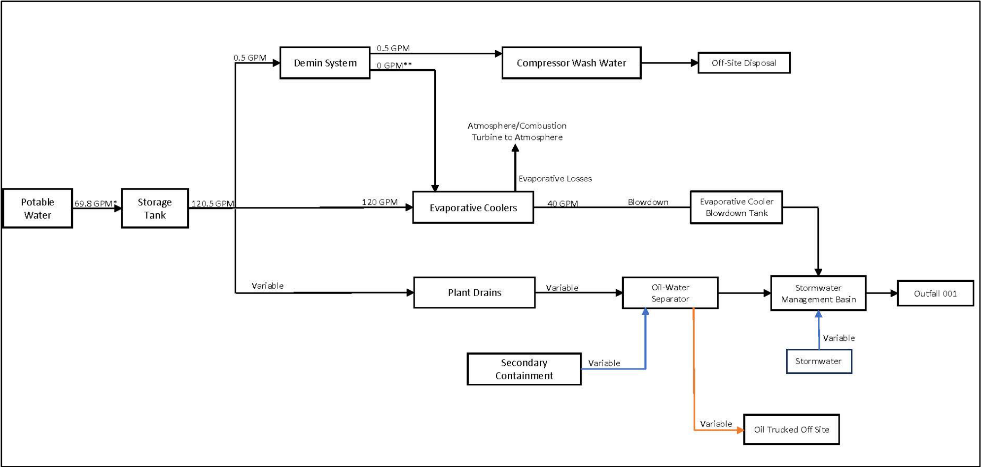
Figure 3: Water Balance Diagram
