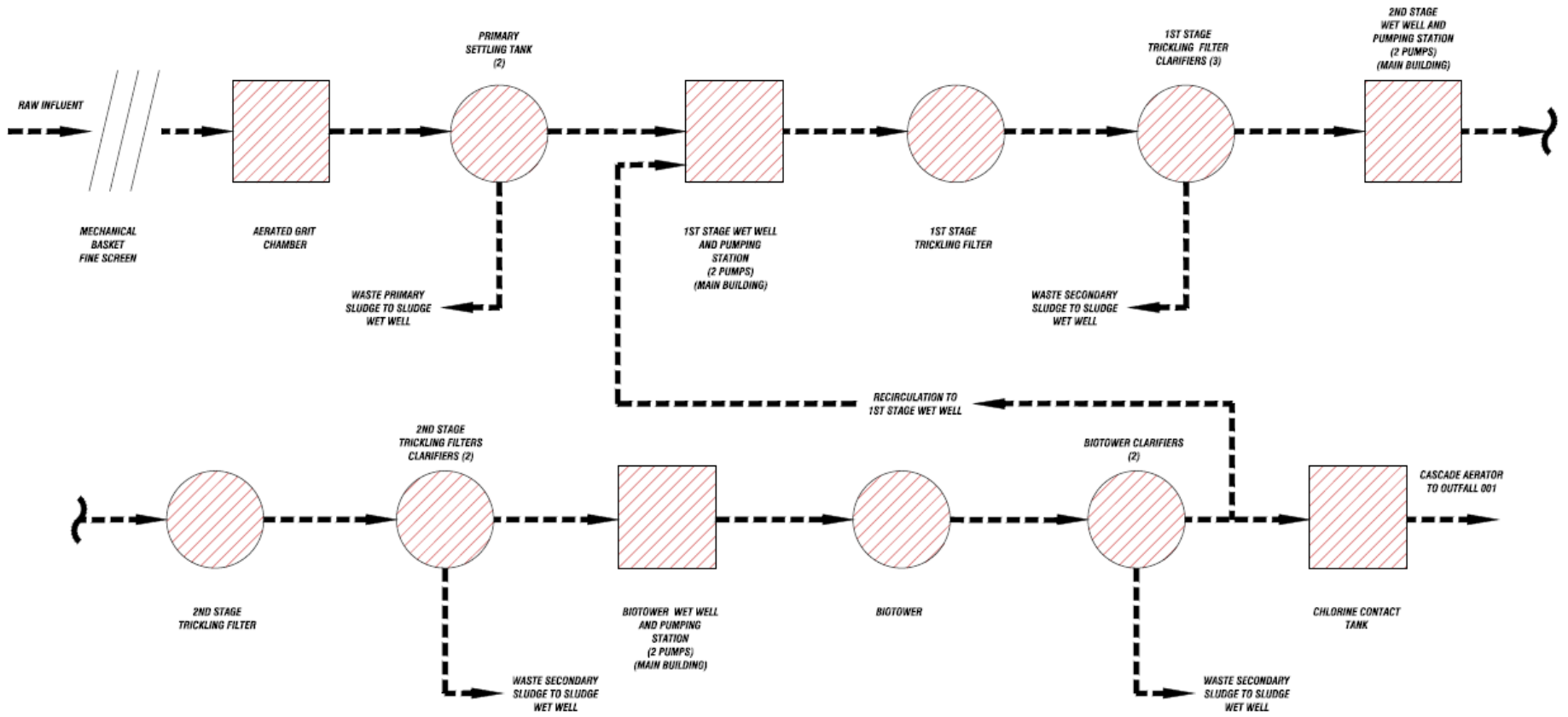
EX. PROCESS FLOW SCHEMATIC
