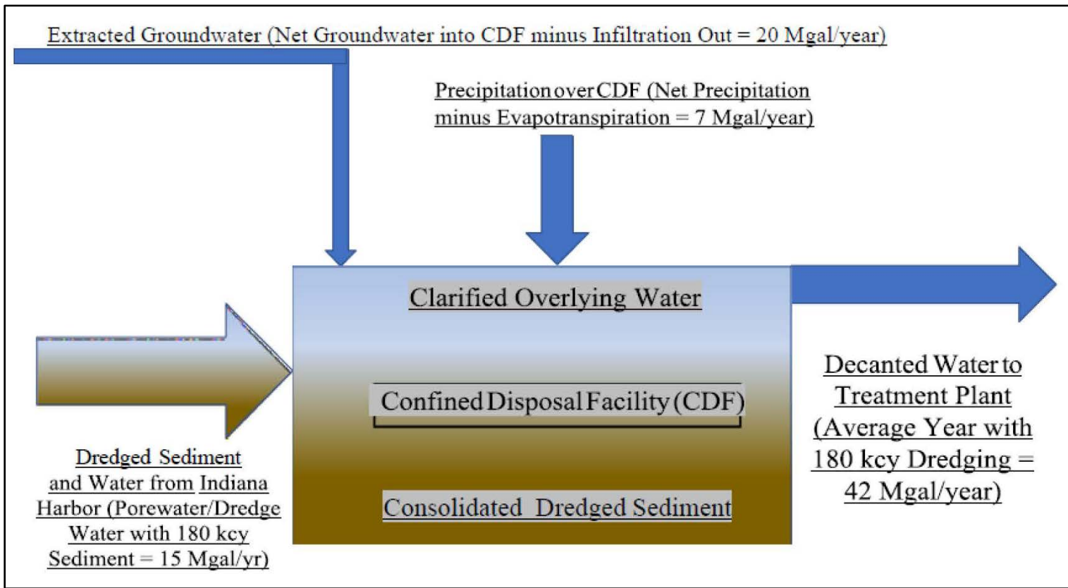
Figure 6: Confined Disposal Facility Flow to Package WWTP
