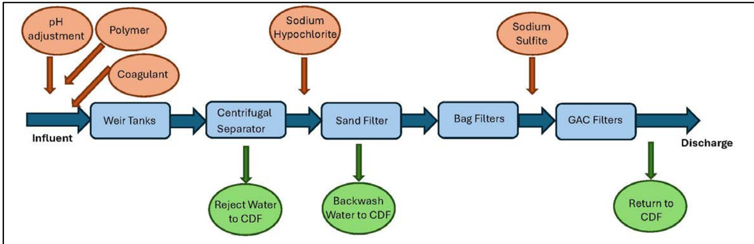
Figure 7: Package WWTP Flow to Outfall 001
