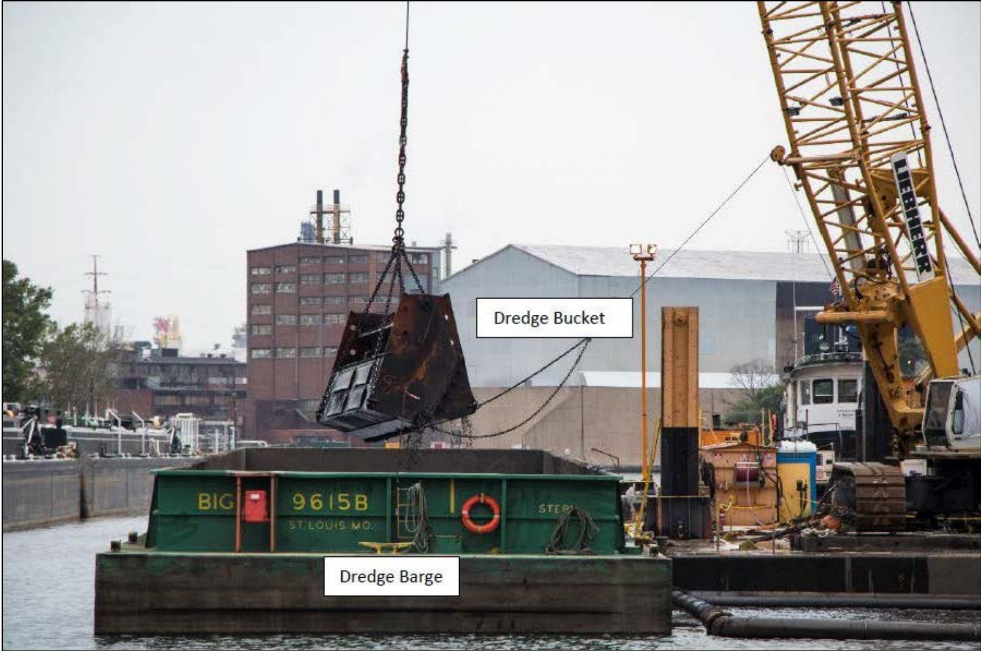
Figure 3 – Mechanical Dredging
