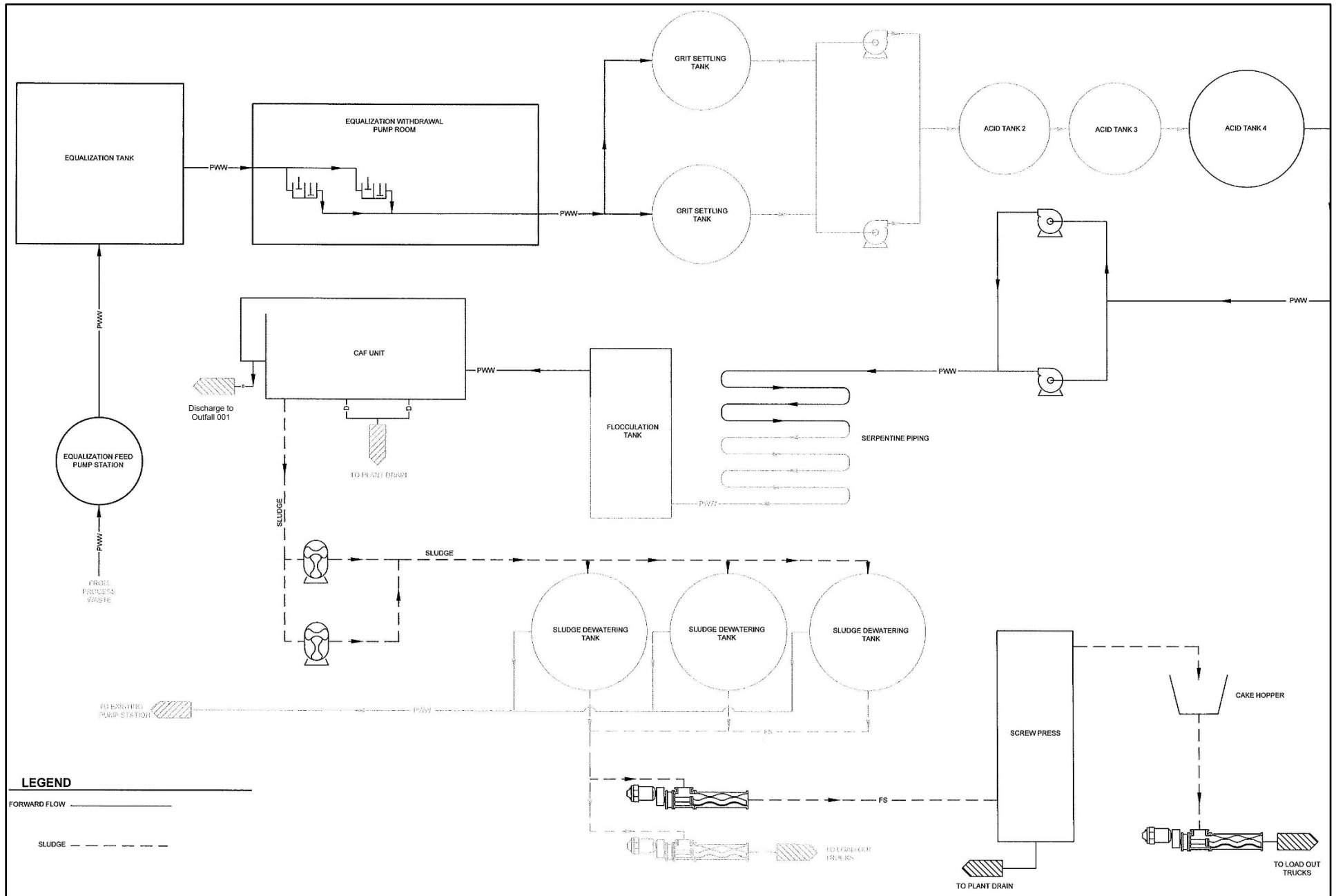
Figure 1: Flow Diagram
