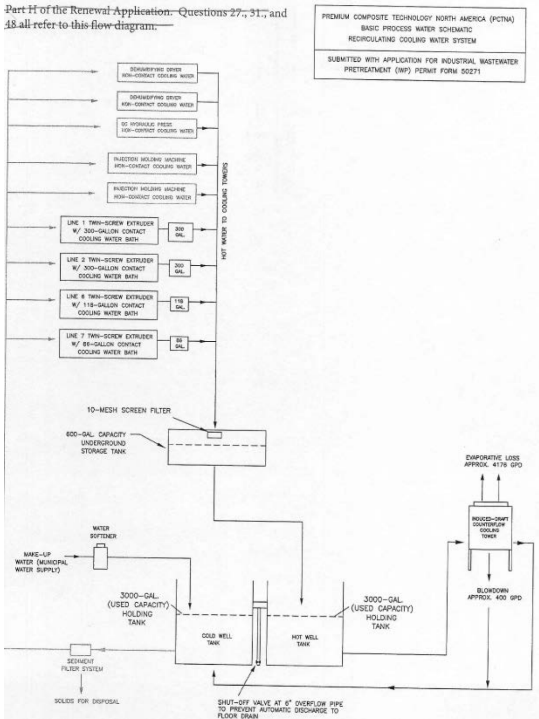
Figure 1: Flow Diagram
