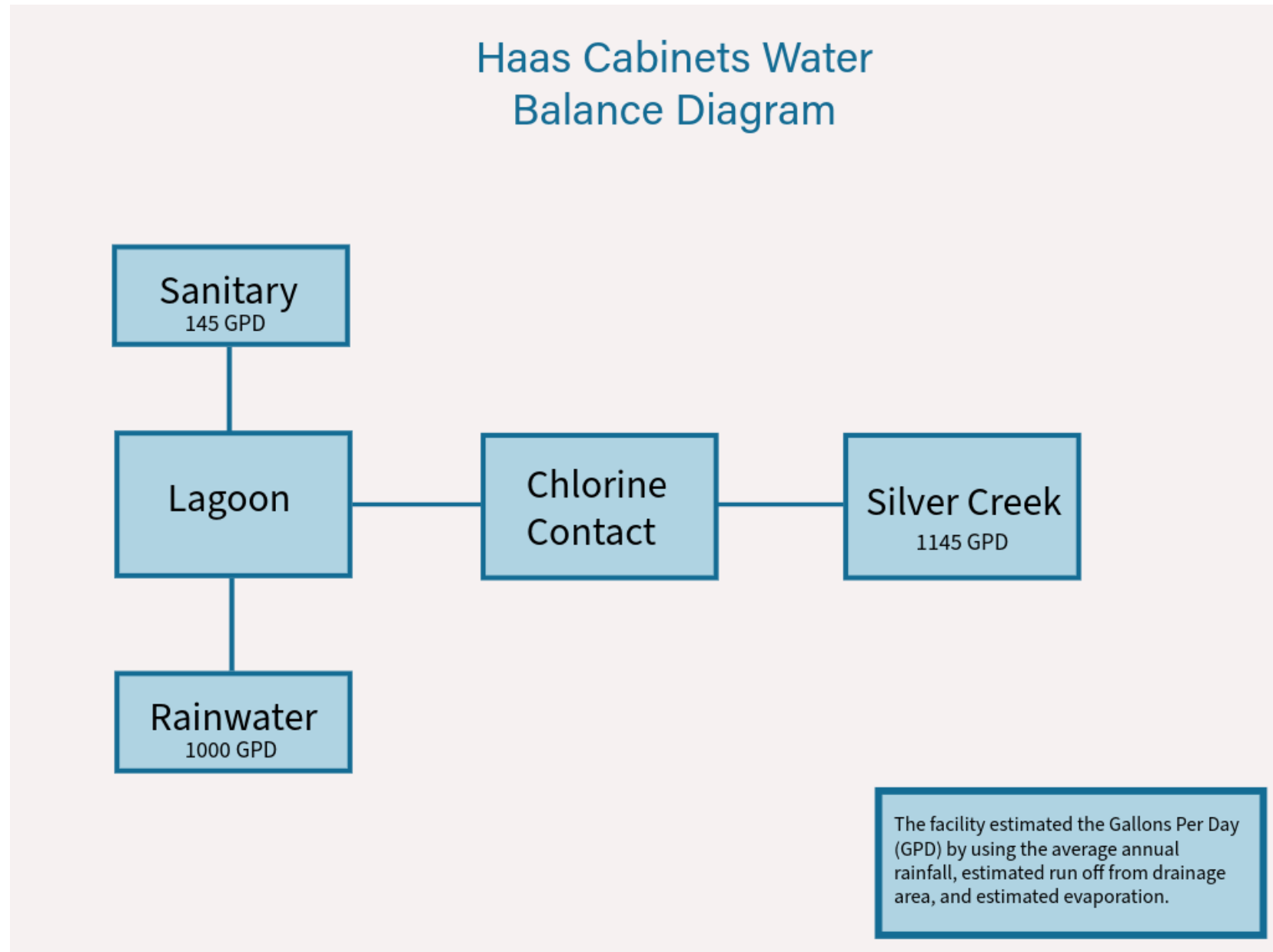
Figure 2: Water Balance Diagram
