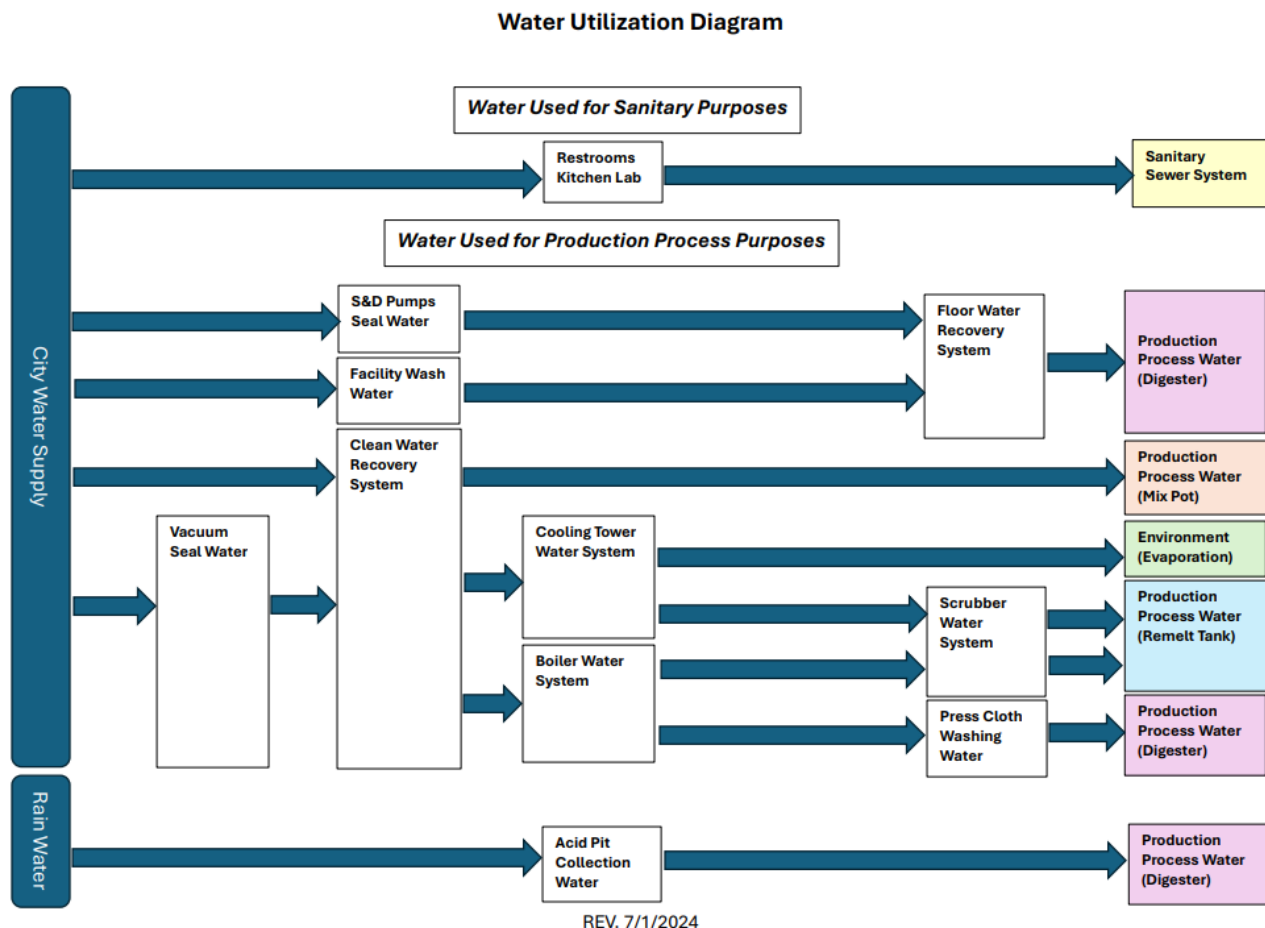
Figure 2: Water Balance Diagram
