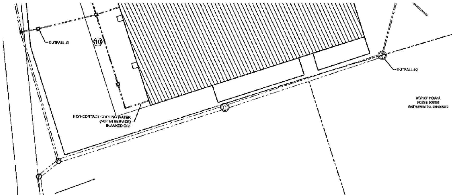
Figure 4: Site Map (zoomed in)
