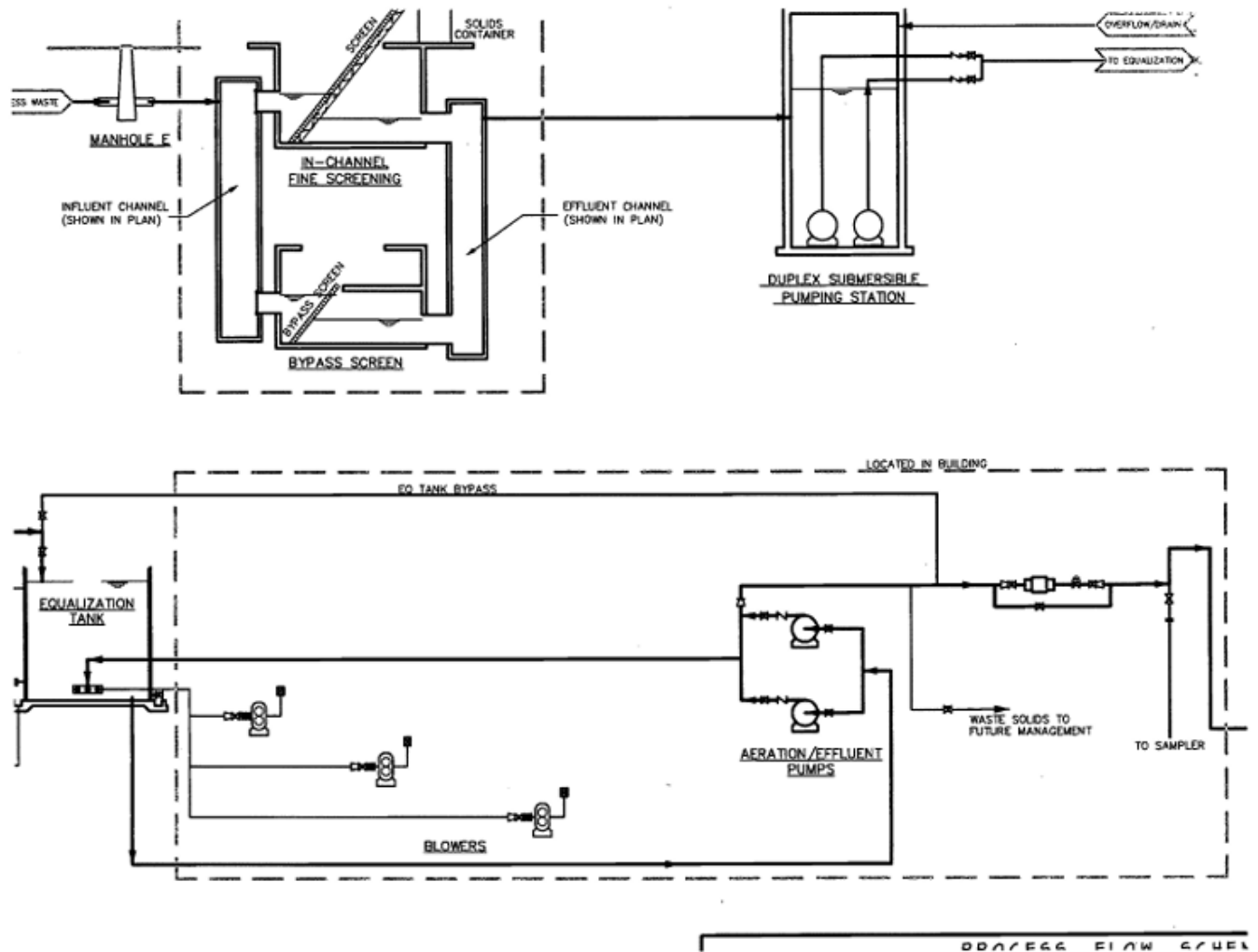
Figure 2: Pretreatment Flow
