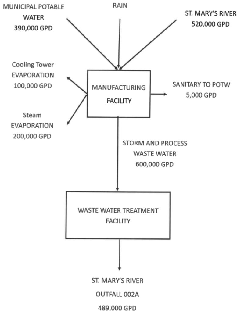
Figure 2: Water Balance Diagram
