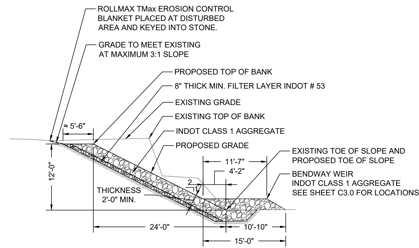
BANK STABILIZATION TYPICAL CROSS SECTION SCALE: 1" = 10'
