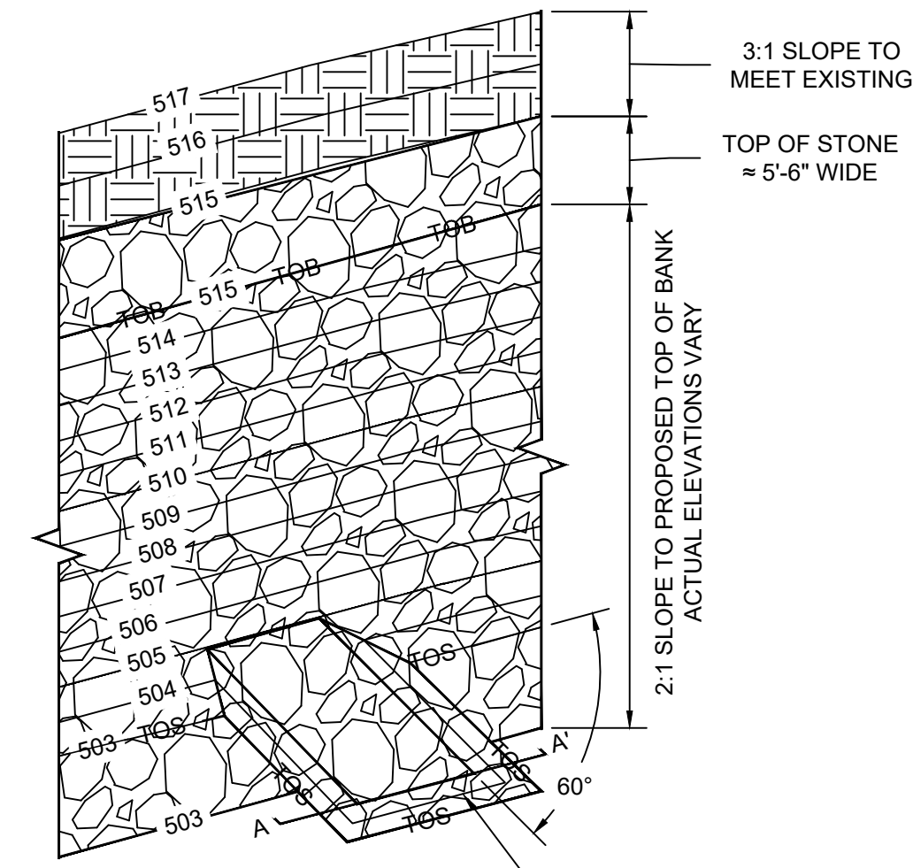
BENDWAY WEIR PLAN SCALE: NOT TO SCALE
