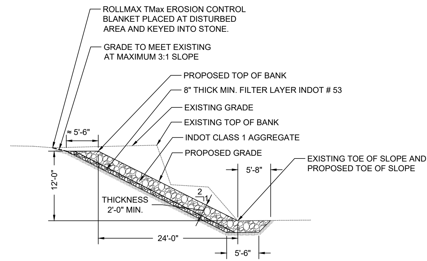
BANK STABILIZATION TYPICAL CROSS SECTION SCALE: 1" = 10'
