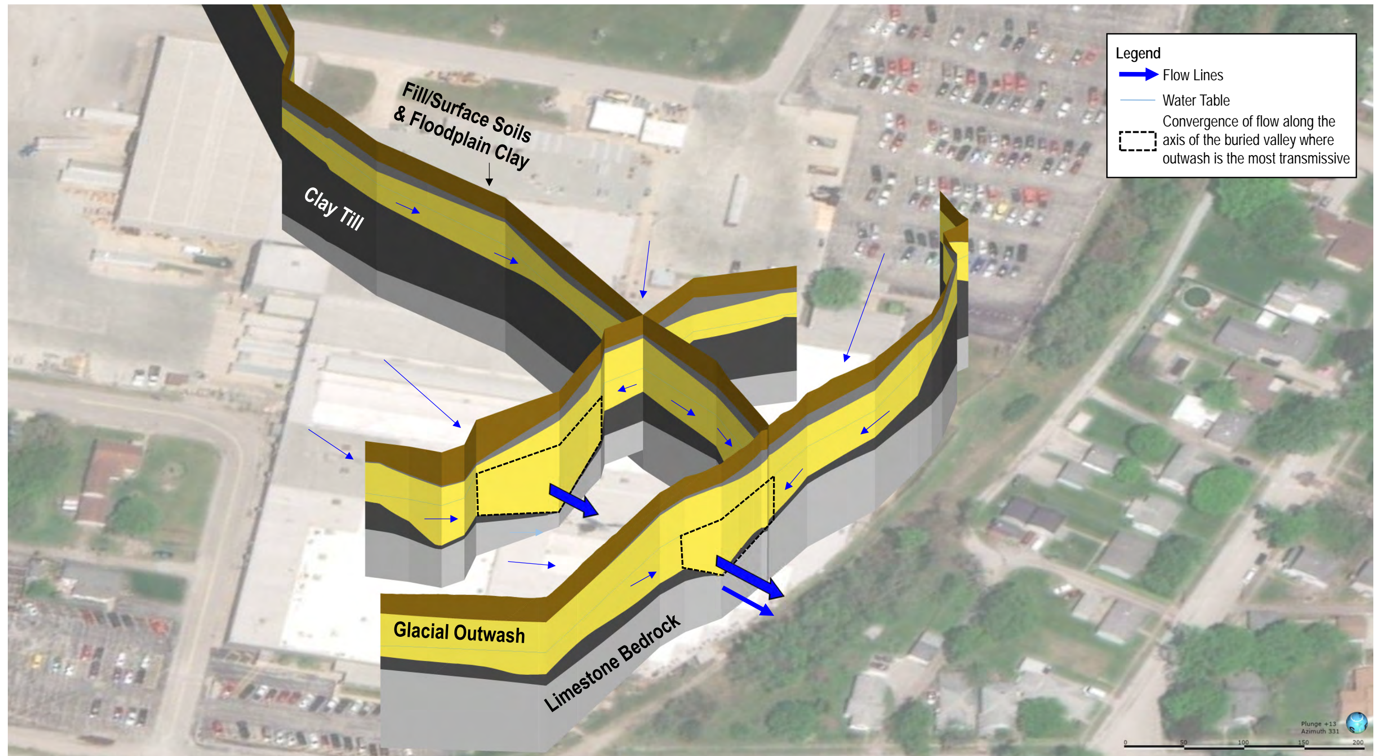
Figure 4 Geologic Fence Diagram Schneider Electric Peru, IN
