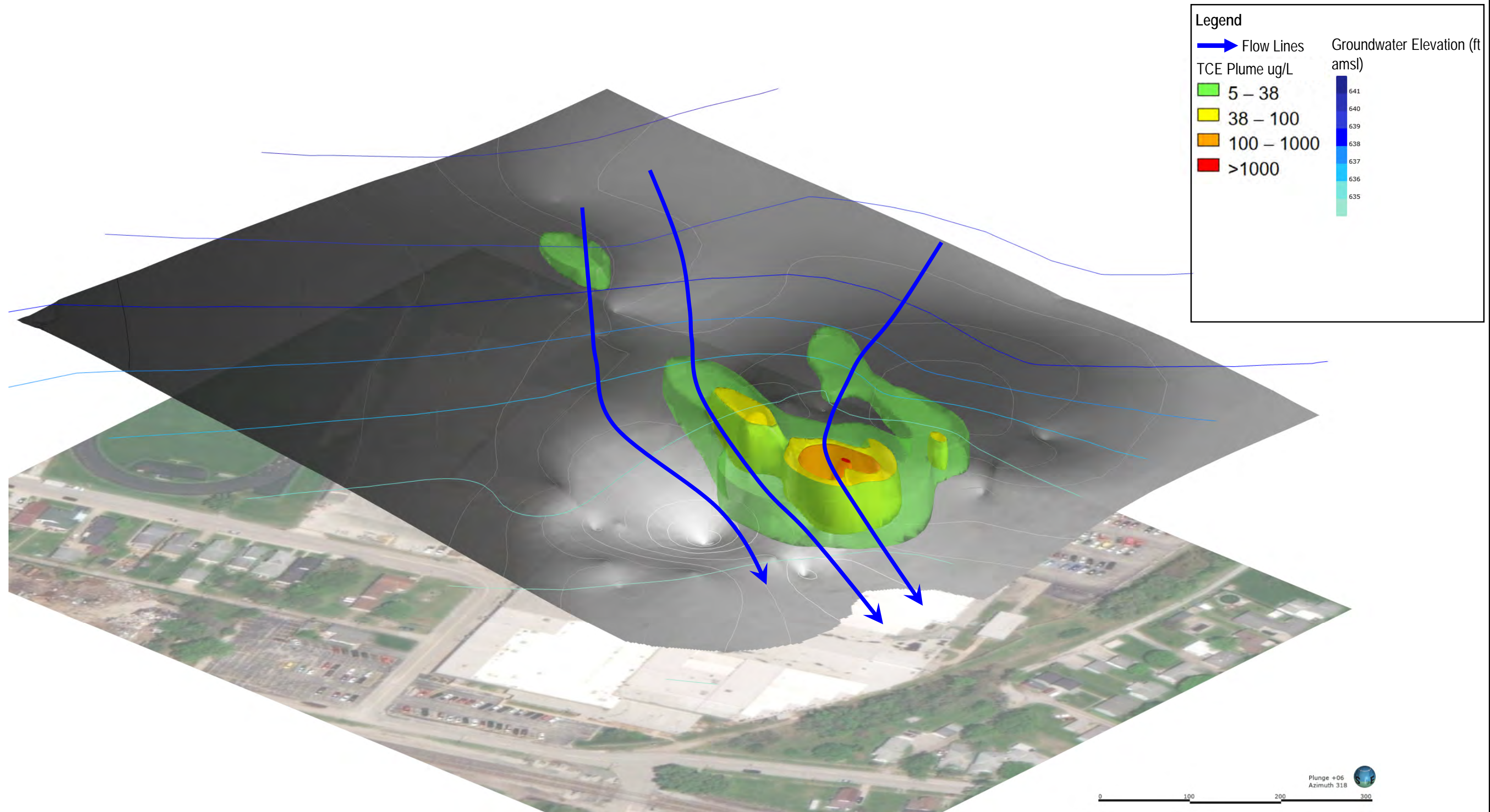
Figure 11 3D TCE Plume and Top of Clay Till Concept Schneider Electric Peru, IN
