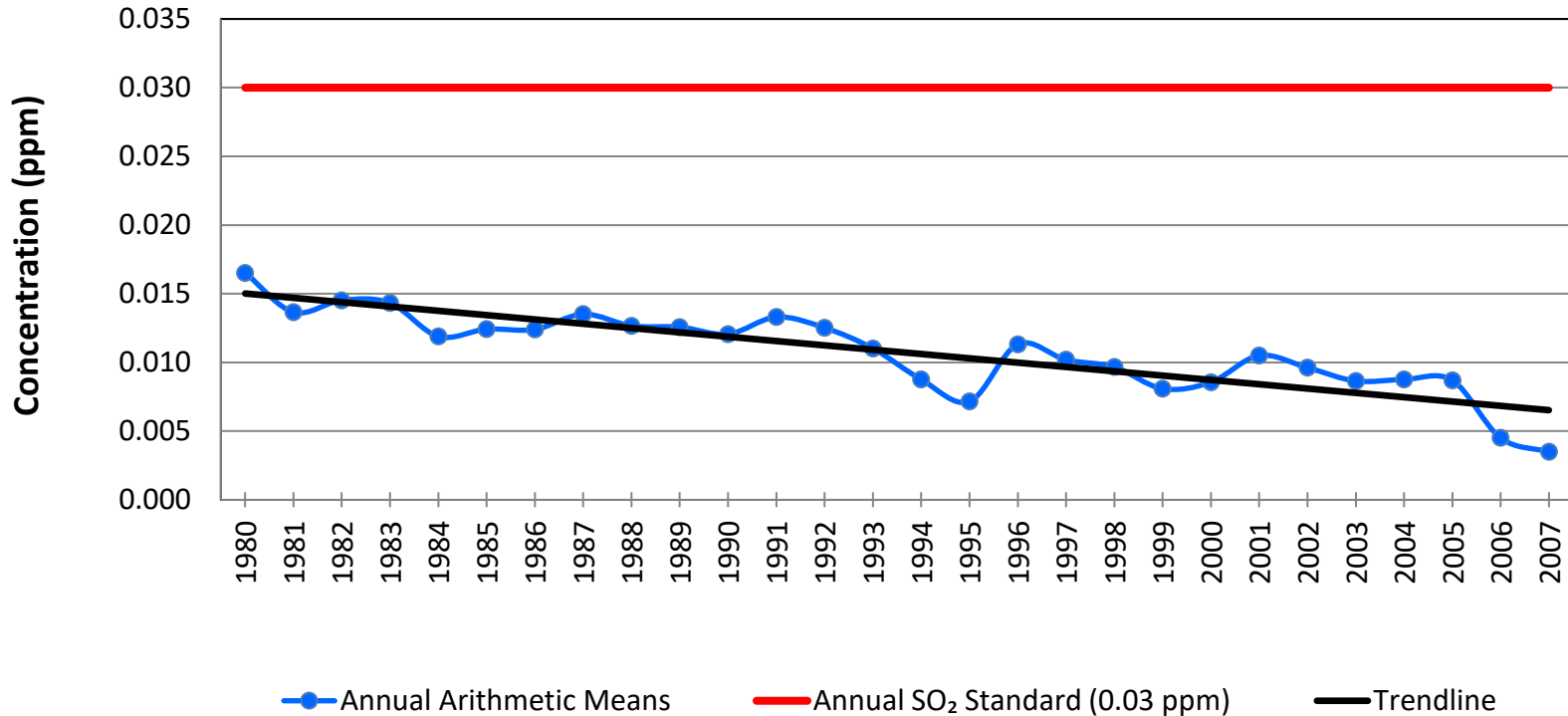
Annual Arithmetic Mean SO 2 Values Central Southeast Indiana
