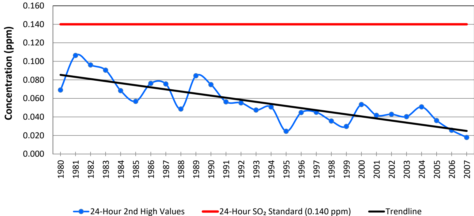
24-Hour SO 2 2nd High Values Central Southeast Indiana
