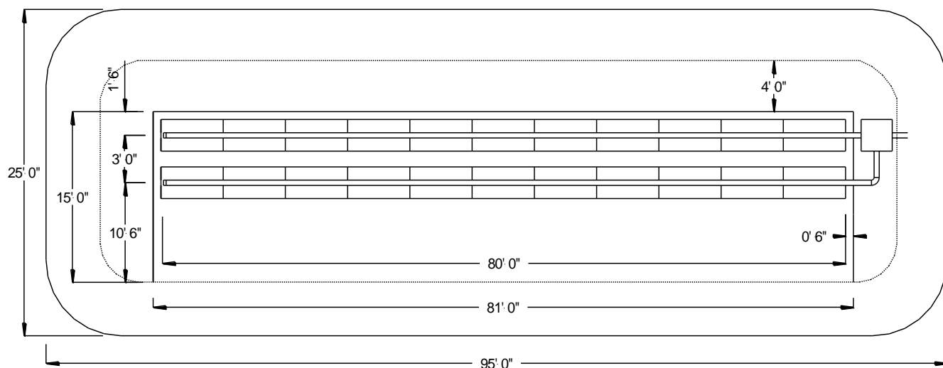
FIGURE 25: PLAN VIEW – 450 GPD – A42 – BED SYSTEM – 0.5% - 6% SLOPE
