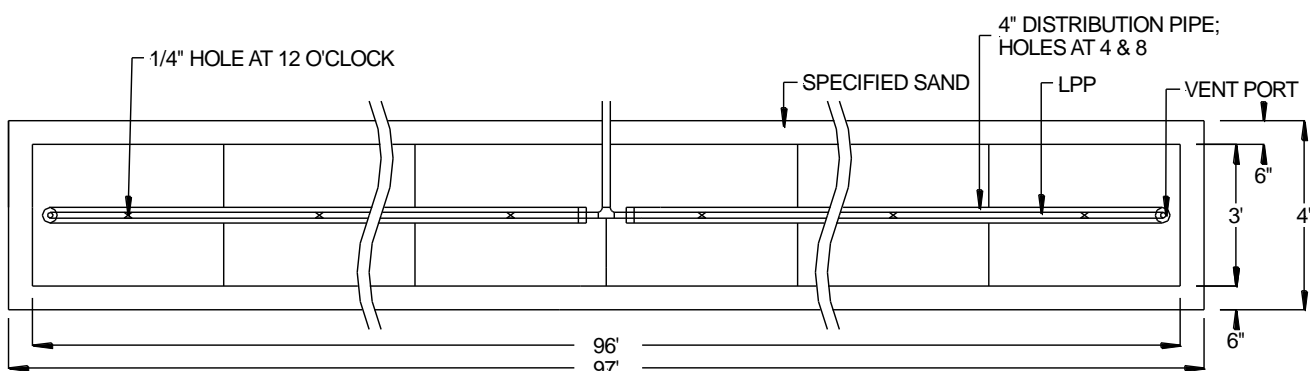
FIGURE 20: PLAN VIEW – 450 GPD – APPLICATION AREA MOUND SYSTEM
