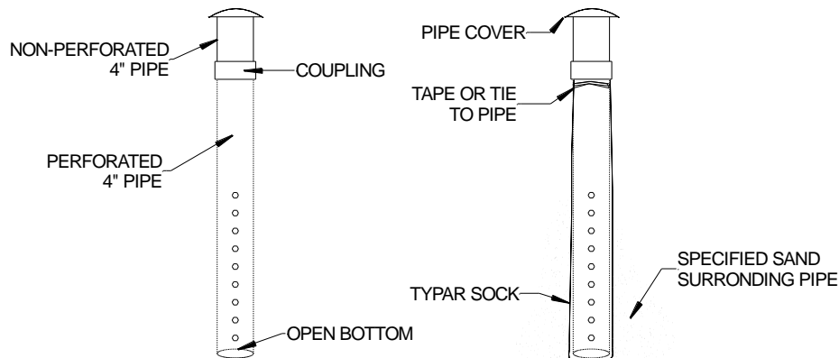
FIGURE 32: MONITORING WELL FOR SAND-SOIL INTERFACE
