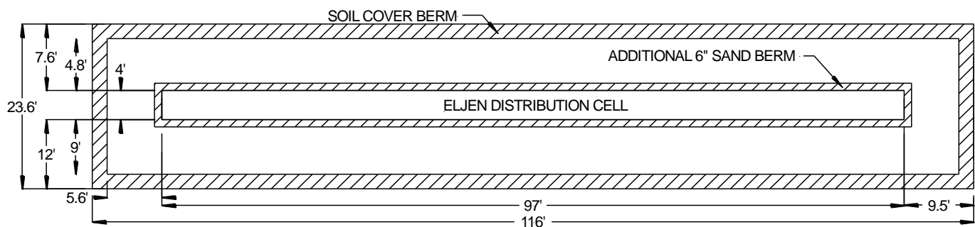
FIGURE 20: PLAN VIEW – 450 GPD – APPLICATION AREA MOUND SYSTEM
