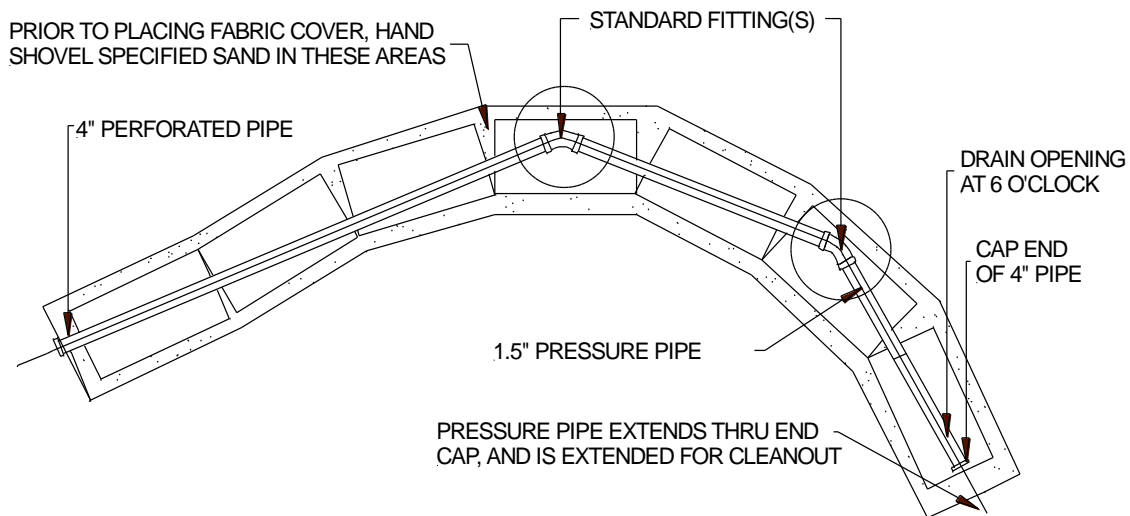
FIGURE 29: CONTOURED TRENCH INSTALLATION
