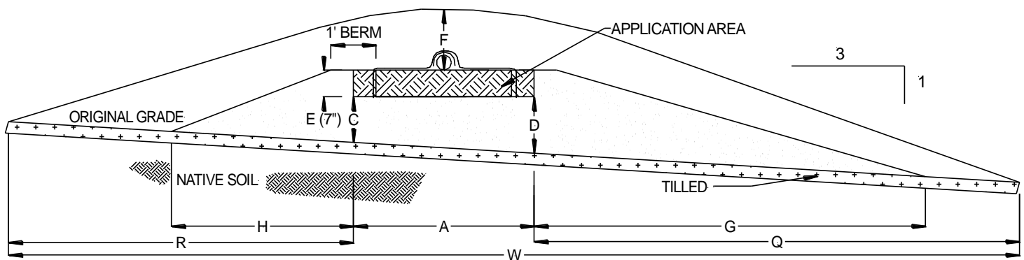
FIGURE 17: PLAN VIEW – MOUND SYSTEM
