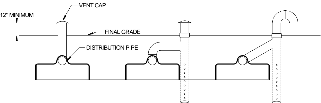
FIGURE 35: COMBINATION VENT/MONITORING WELL FOR SAND-SOIL INTERFACE
