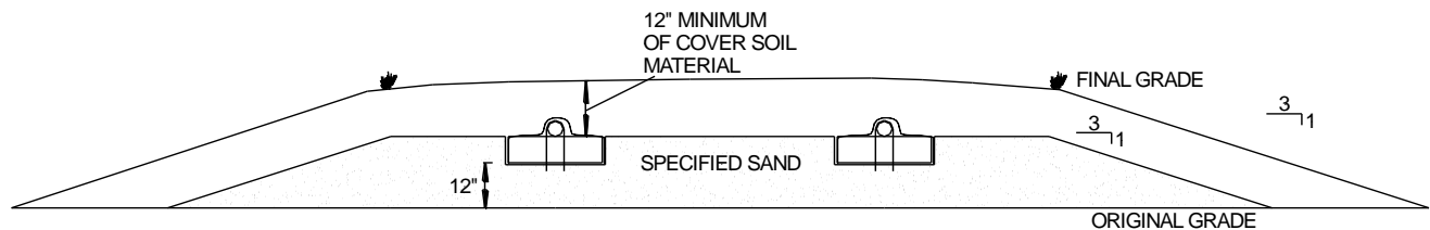
FIGURE 21: ABOVE GRADE BED CROSS SECTION
