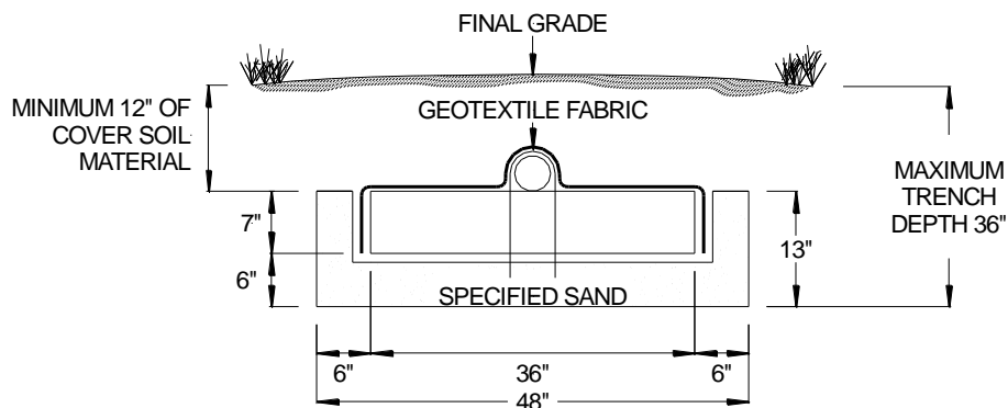
FIGURE 4: SUBSURFACE B43 SINGLE LATERAL BED CROSS SECTION
