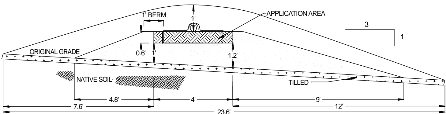
FIGURE 19: PLAN VIEW – MOUND SYSTEM
