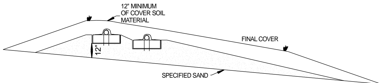
FIGURE 24: SLOPED ABOVE GRADE BED CROSS SECTION
