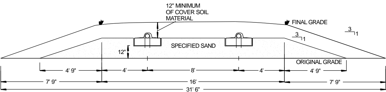
FIGURE 23: CROSS SECTION VIEW – 600 GPD – A42 – BED SYSTEM – \leq 0.5\% SLOPE
