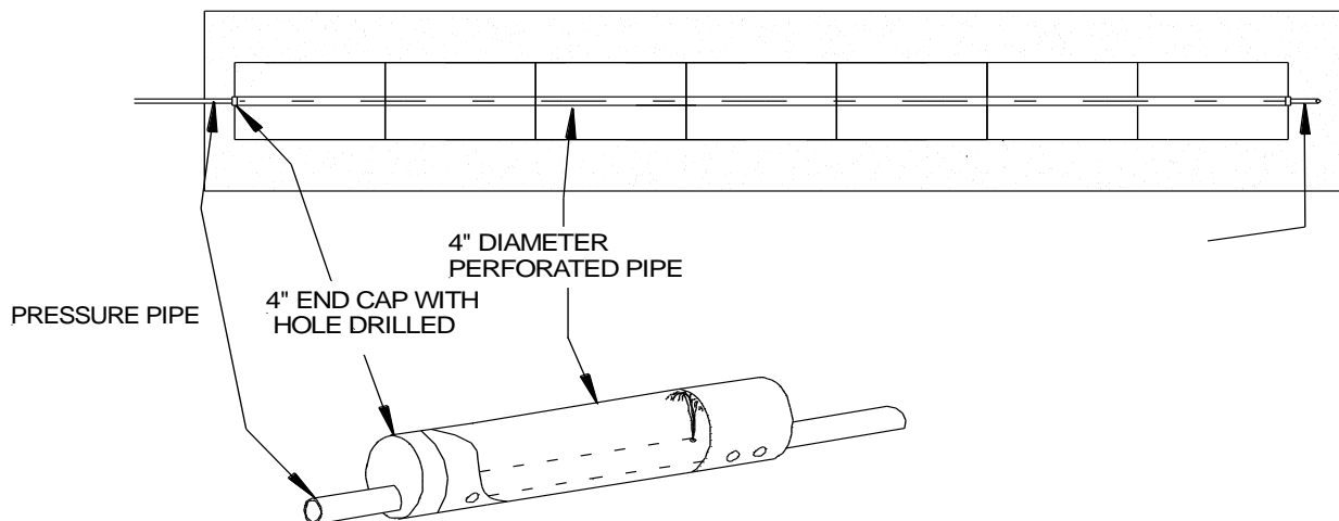
FIGURE 27: PRESSURE PIPE PLACEMENT
