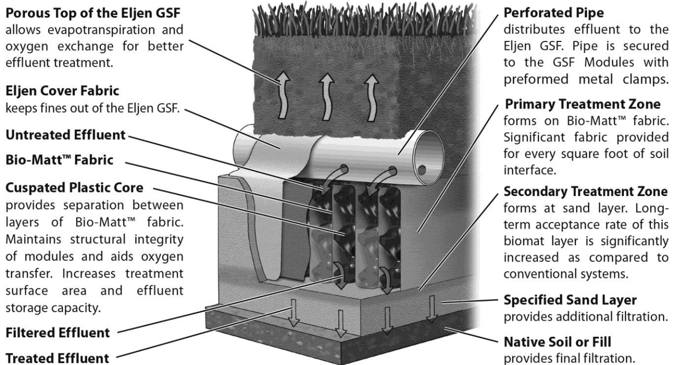
FIGURE 1: GSF SYSTEM OPERATION
