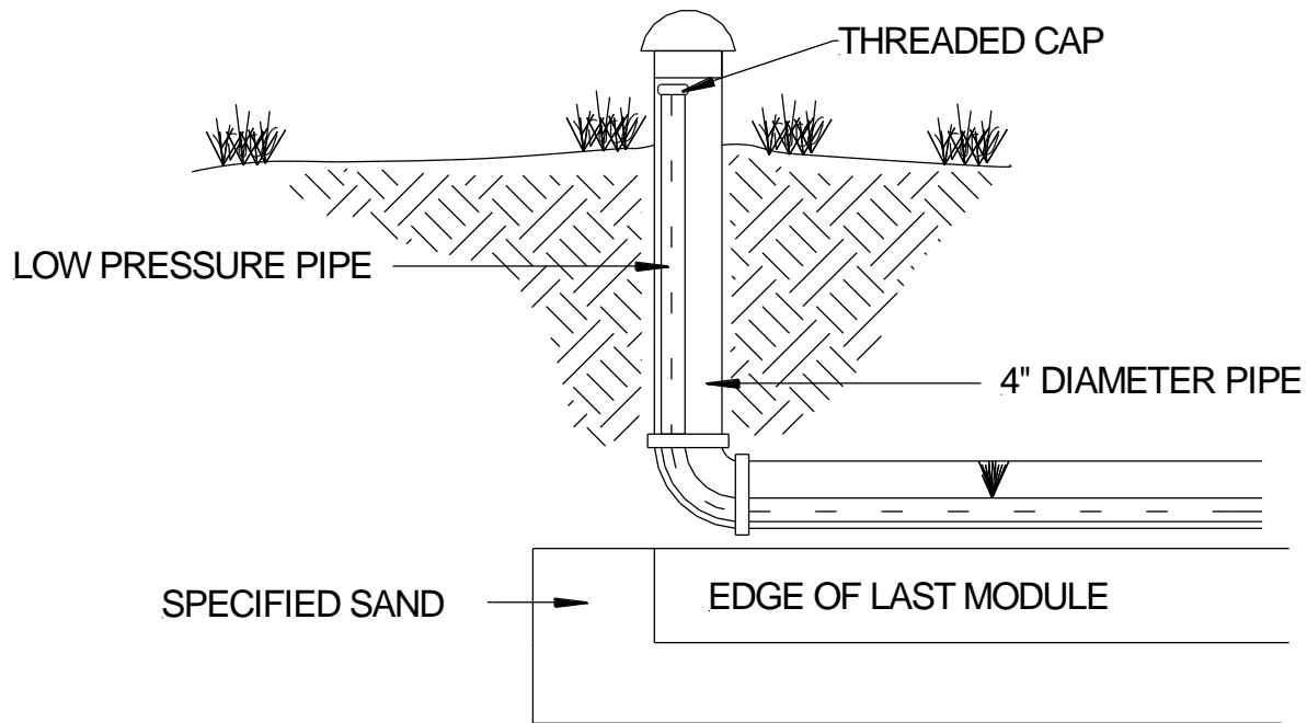
FIGURE 31: GSF VENT WITH PRESSURE DISTRIBUTION
