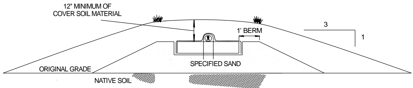
FIGURE 15: ELEVATED SAND MOUND CROSS SECTION
