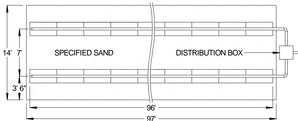
FIGURE 9: PLAN VIEW – 600GPD – A42 – BED SYSTEM – ≤ 0.5% SLOPE
