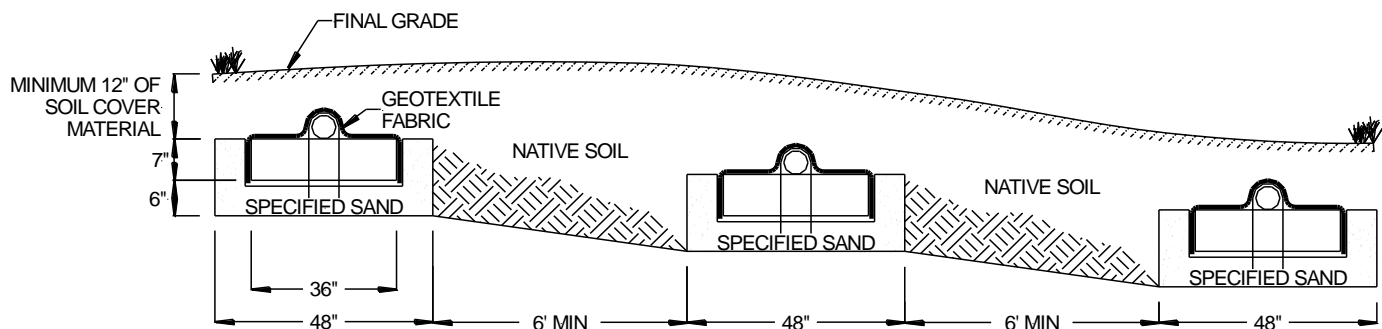
FIGURE 7: SECTION VIEW – B43 – SINGLE LATERAL BED SYSTEM – 0.5 – 15% SLOPE
