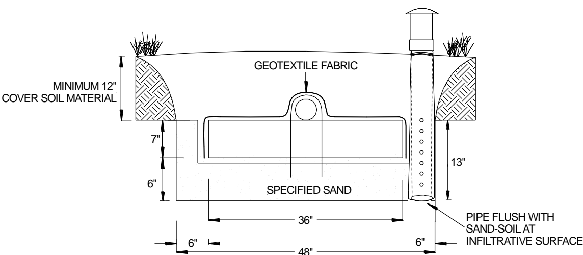
FIGURE 33: OBSERVATION PORT INSTALLED NEXT TO MODULE
