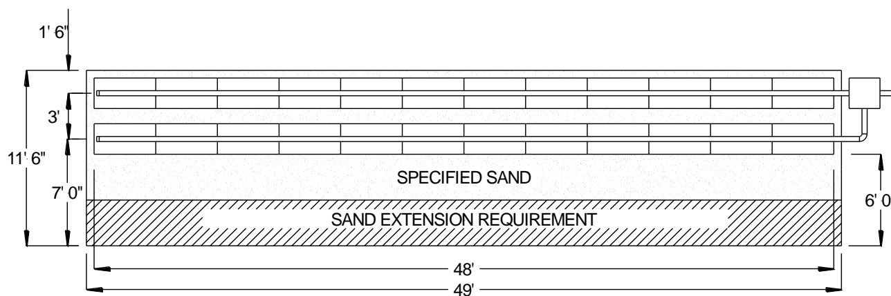
FIGURE 13: PLAN VIEW – 450 GPD – A42 – BED SYSTEM – 0.5 – 15% SLOPE
