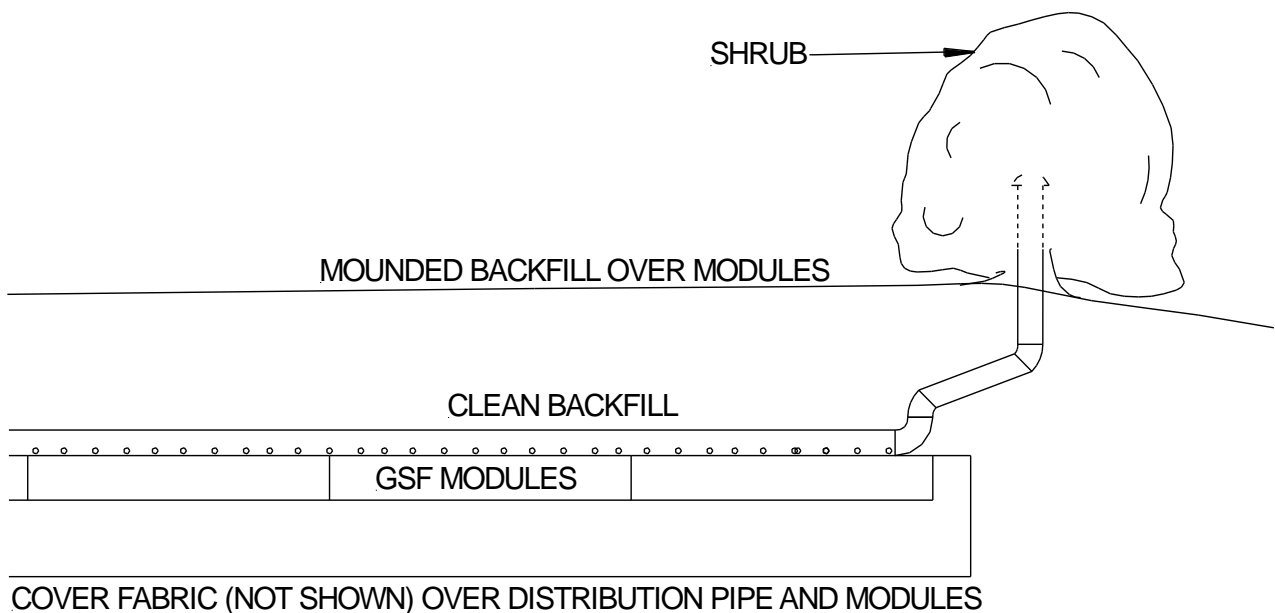
FIGURE 30: GSF WITH 4" VENT EXTENDED TO CONVENIENT LOCATION
