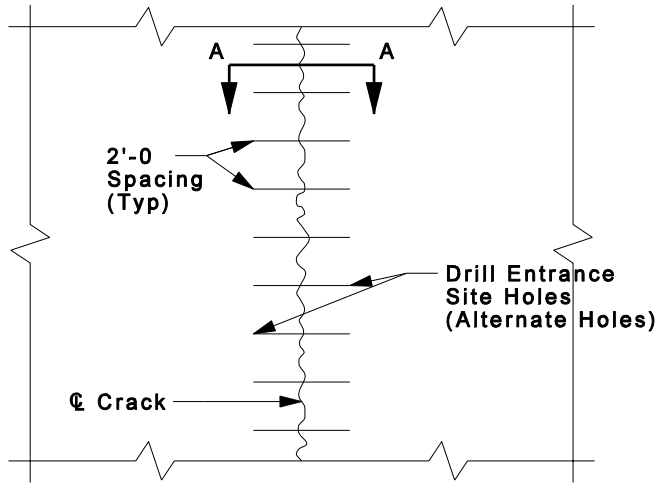
Longitudinal or Transverse Crack
