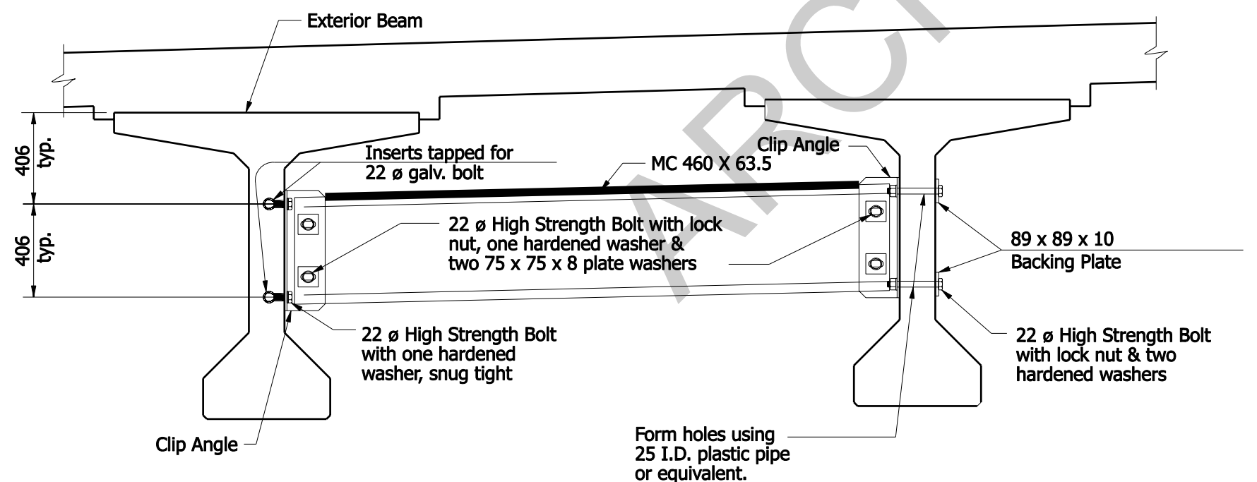
INTERMEDIATE DIAPHRAGM Typical for Skewed Structure
