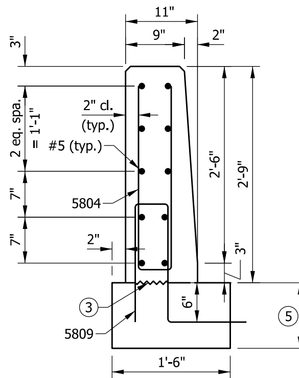
SECTION C-C
