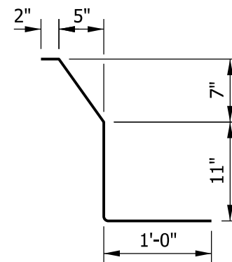
5816 x 2'-10"
