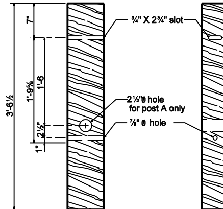
SIDE FRONT BCT TIMBER POST
