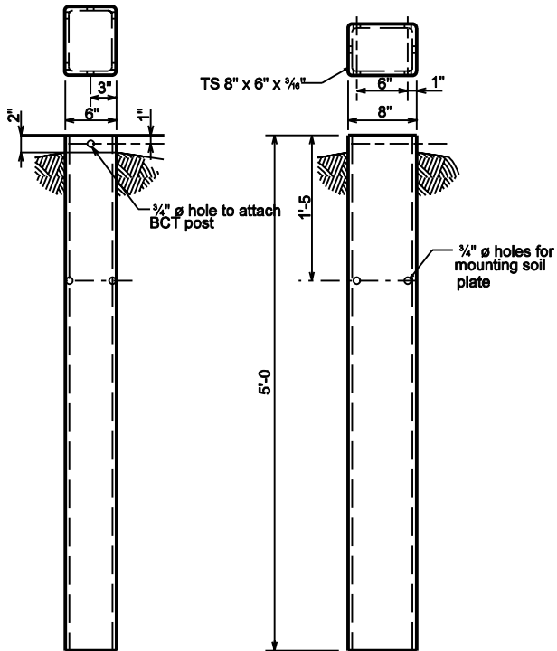
FRONT SIDE GALVANIZED STEEL FOUNDATION TUBE
