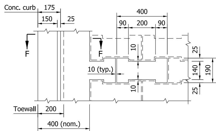
PLAN - PRECAST CONCRETE RIPRAP (Type A shown)
