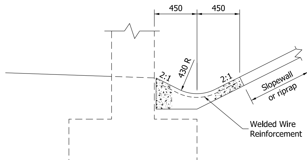
SECTION THROUGH PAVED DITCH AT TOE OF SLOPE (See layout on plans for location of paved ditch)
