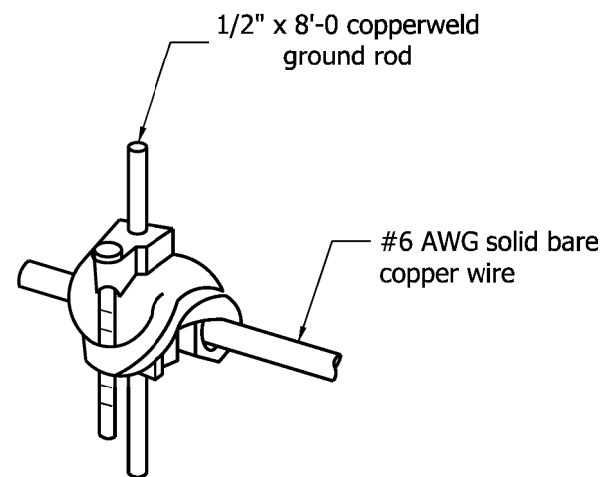
Grounding grid connector
