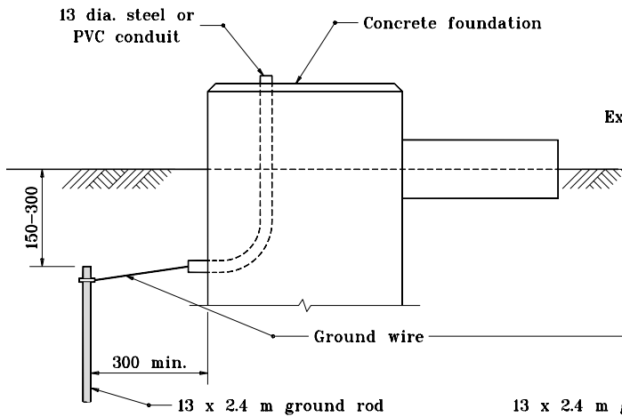
TYPICAL DETAIL GROUND ROD IN EARTH
