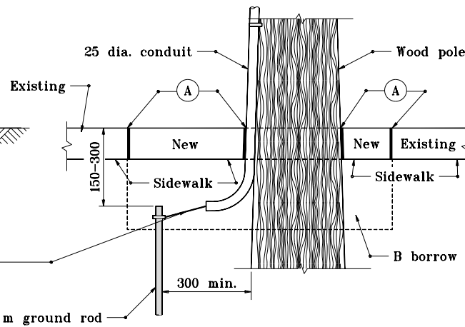
TYPICAL DETAIL GROUND ROD IN SIDEWALK
