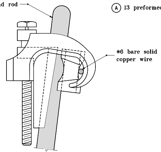
GROUNDING GRID
