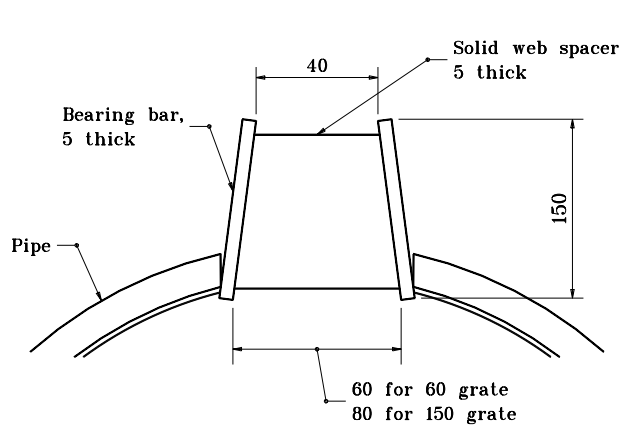
SECTION A-A STANDARD GRATE DETAIL
