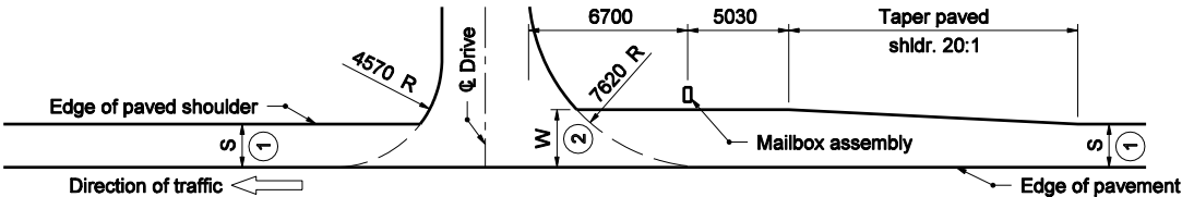
COMBINATION MAILBOX APPROACH & DRIVE (Mailbox located before drive)
